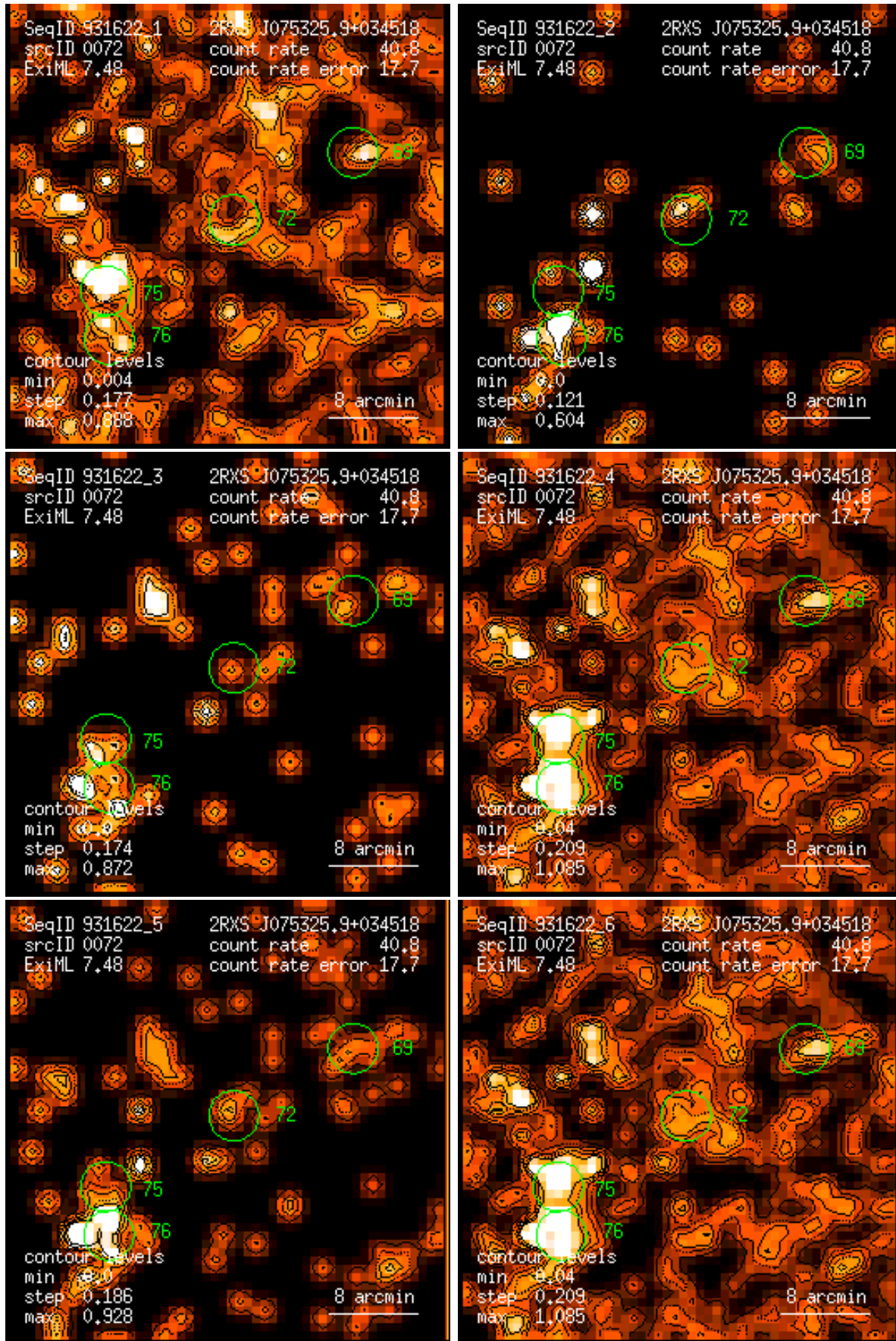
Figure 72: RASS 931622: detection 0072: band rate images, Gaussian filter: (1) PSPC channels 11 – 41, (2) 52 – 90, (3) 91 – 201, (4) 11 – 235, (5) 52 – 201, (6) 11 – 201. Broad band rates in counts/ks. Band rate contour levels in counts/ks/arcmin 2 .
