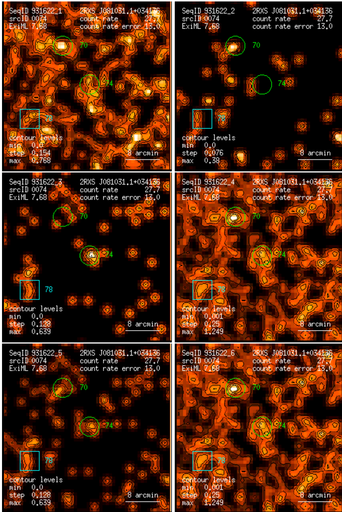
Figure 74: RASS 931622: detection 0074: band rate images, Gaussian filter: (1) PSPC channels 11 – 41, (2) 52 – 90, (3) 91 – 201, (4) 11 – 235, (5) 52 – 201, (6) 11 – 201. Broad band rates in counts/ks. Band rate contour levels in counts/ks/arcmin 2 .
