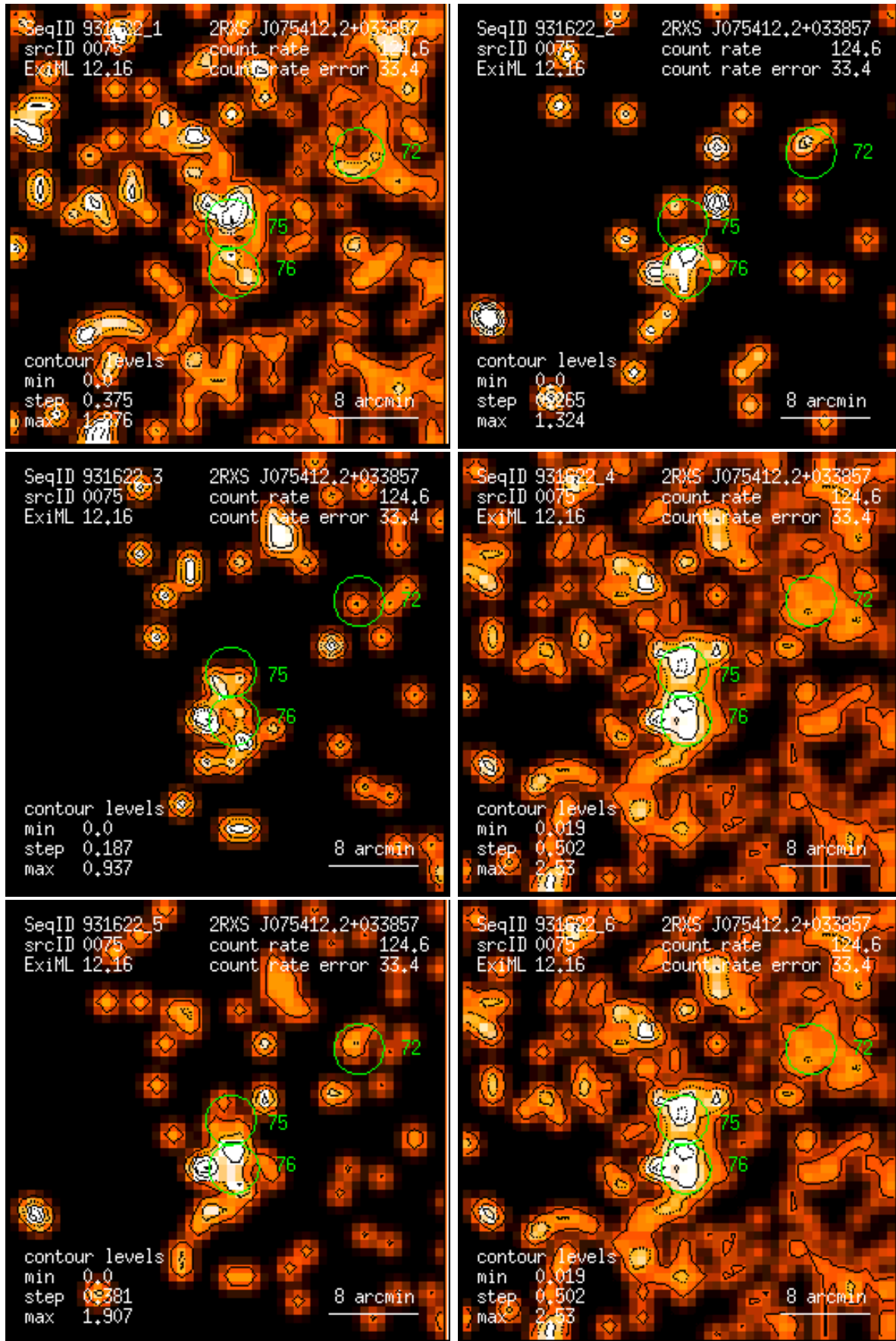
Figure 75: RASS 931622: detection 0075: band rate images, Gaussian filter: (1) PSPC channels 11 – 41, (2) 52 – 90, (3) 91 – 201, (4) 11 – 235, (5) 52 – 201, (6) 11 – 201. Broad band rates in counts/ks. Band rate contour levels in counts/ks/arcmin 2 .
