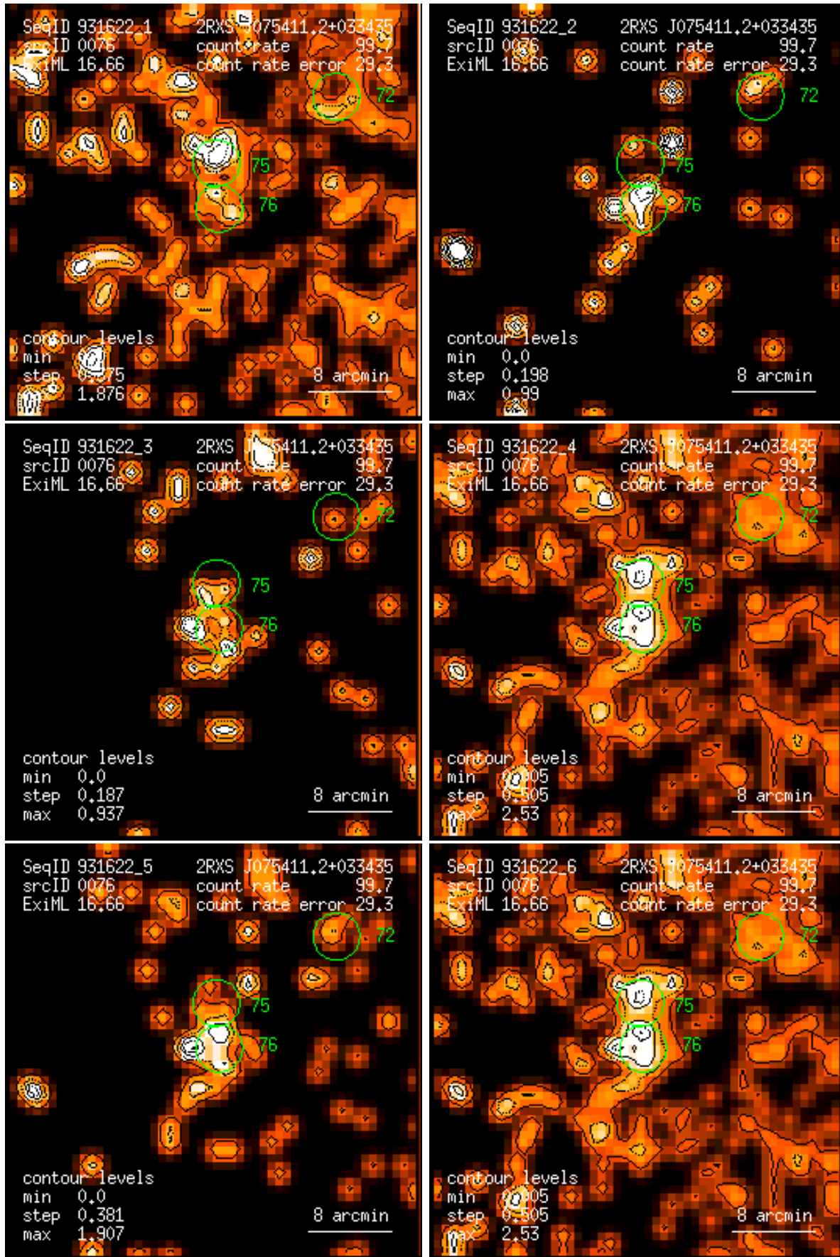
Figure 76: RASS 931622: detection 0076: band rate images, Gaussian filter: (1) PSPC channels 11 – 41, (2) 52 – 90, (3) 91 – 201, (4) 11 – 235, (5) 52 – 201, (6) 11 – 201. Broad band rates in counts/ks. Band rate contour levels in counts/ks/arcmin 2 .
