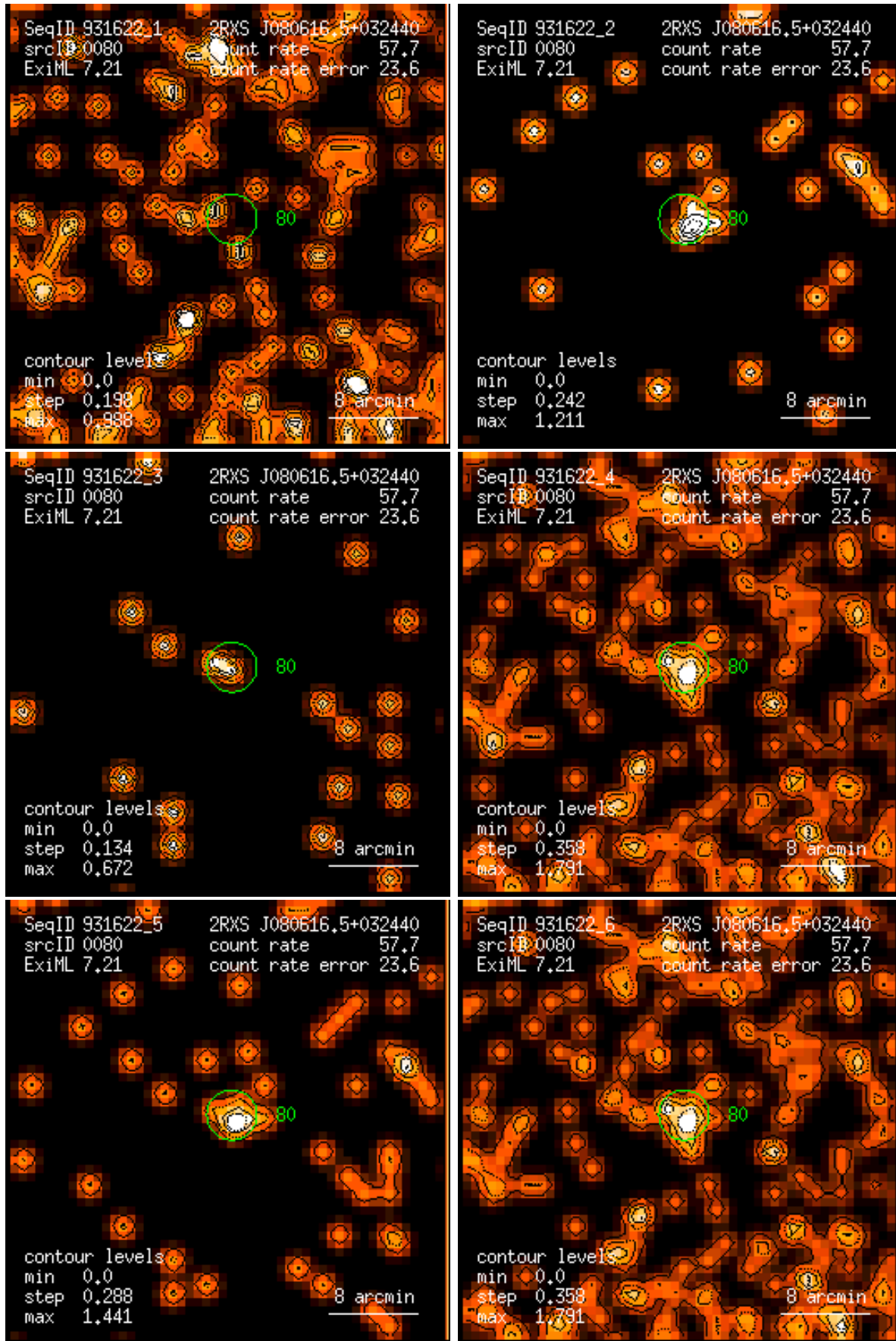
Figure 80: RASS 931622: detection 0080: band rate images, Gaussian filter: (1) PSPC channels 11 – 41, (2) 52 – 90, (3) 91 – 201, (4) 11 – 235, (5) 52 – 201, (6) 11 – 201. Broad band rates in counts/ks. Band rate contour levels in counts/ks/arcmin 2 .
