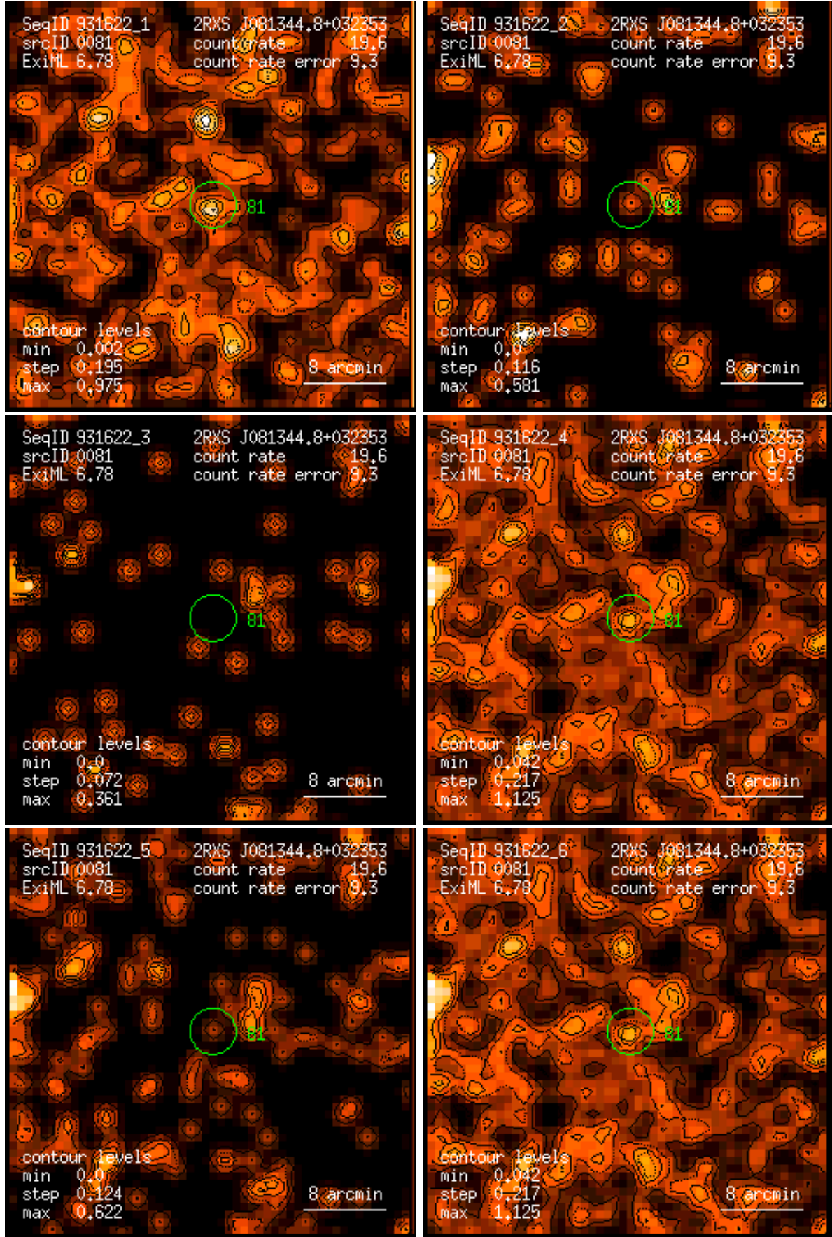
Figure 81: RASS 931622: detection 0081: band rate images, Gaussian filter: (1) PSPC channels 11 – 41, (2) 52 – 90, (3) 91 – 201, (4) 11 – 235, (5) 52 – 201, (6) 11 – 201. Broad band rates in counts/ks. Band rate contour levels in counts/ks/arcmin 2 .
