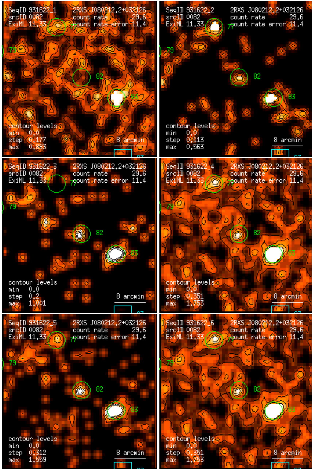
Figure 82: RASS 931622: detection 0082: band rate images, Gaussian filter: (1) PSPC channels 11 – 41, (2) 52 – 90, (3) 91 – 201, (4) 11 – 235, (5) 52 – 201, (6) 11 – 201. Broad band rates in counts/ks. Band rate contour levels in counts/ks/arcmin 2 .
