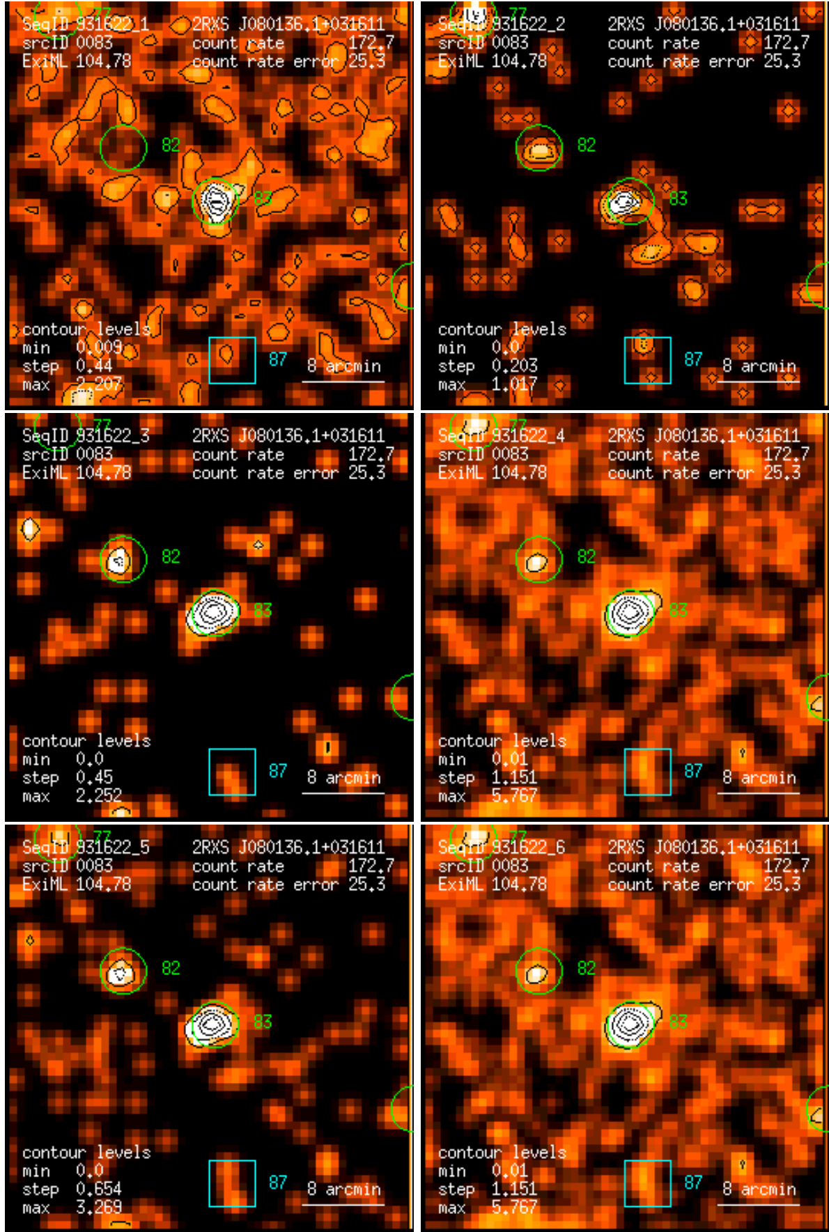
Figure 83: RASS 931622: detection 0083: band rate images, Gaussian filter: (1) PSPC channels 11 – 41, (2) 52 – 90, (3) 91 – 201, (4) 11 – 235, (5) 52 – 201, (6) 11 – 201. Broad band rates in counts/ks. Band rate contour levels in counts/ks/arcmin 2 .
