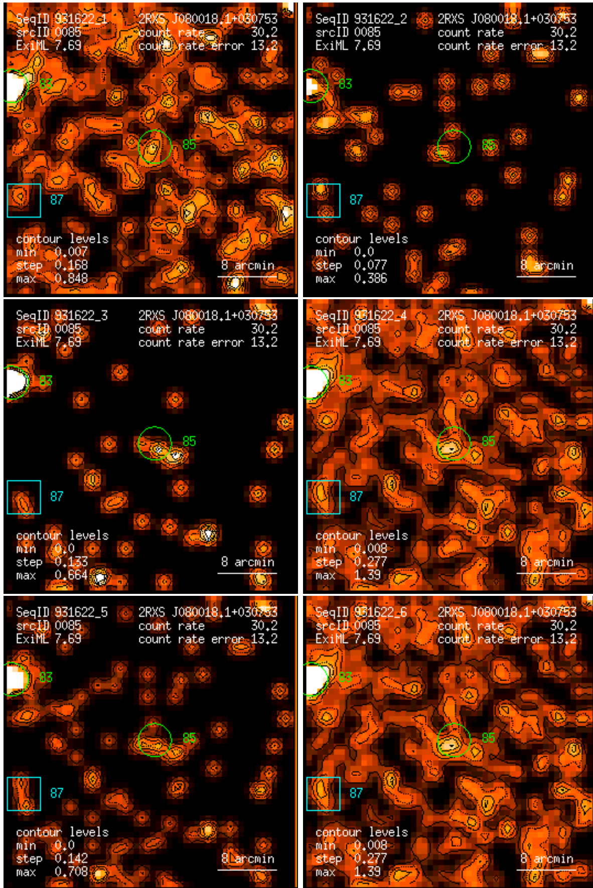
Figure 85: RASS 931622: detection 0085: band rate images, Gaussian filter: (1) PSPC channels 11 – 41, (2) 52 – 90, (3) 91 – 201, (4) 11 – 235, (5) 52 – 201, (6) 11 – 201. Broad band rates in counts/ks. Band rate contour levels in counts/ks/arcmin 2 .
