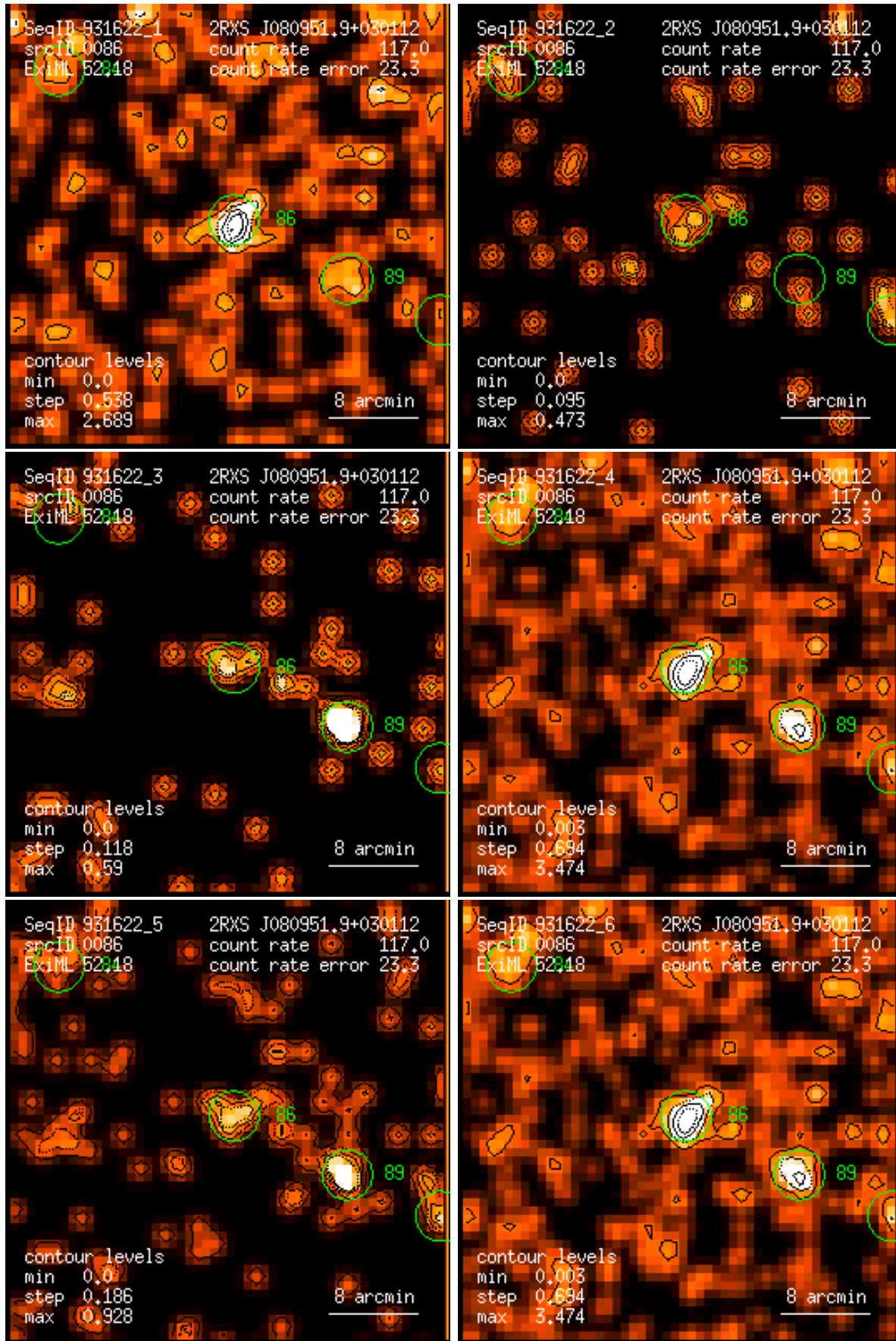
Figure 86: RASS 931622: detection 0086: band rate images, Gaussian filter: (1) PSPC channels 11 – 41, (2) 52 – 90, (3) 91 – 201, (4) 11 – 235, (5) 52 – 201, (6) 11 – 201. Broad band rates in counts/ks. Band rate contour levels in counts/ks/arcmin 2 .
