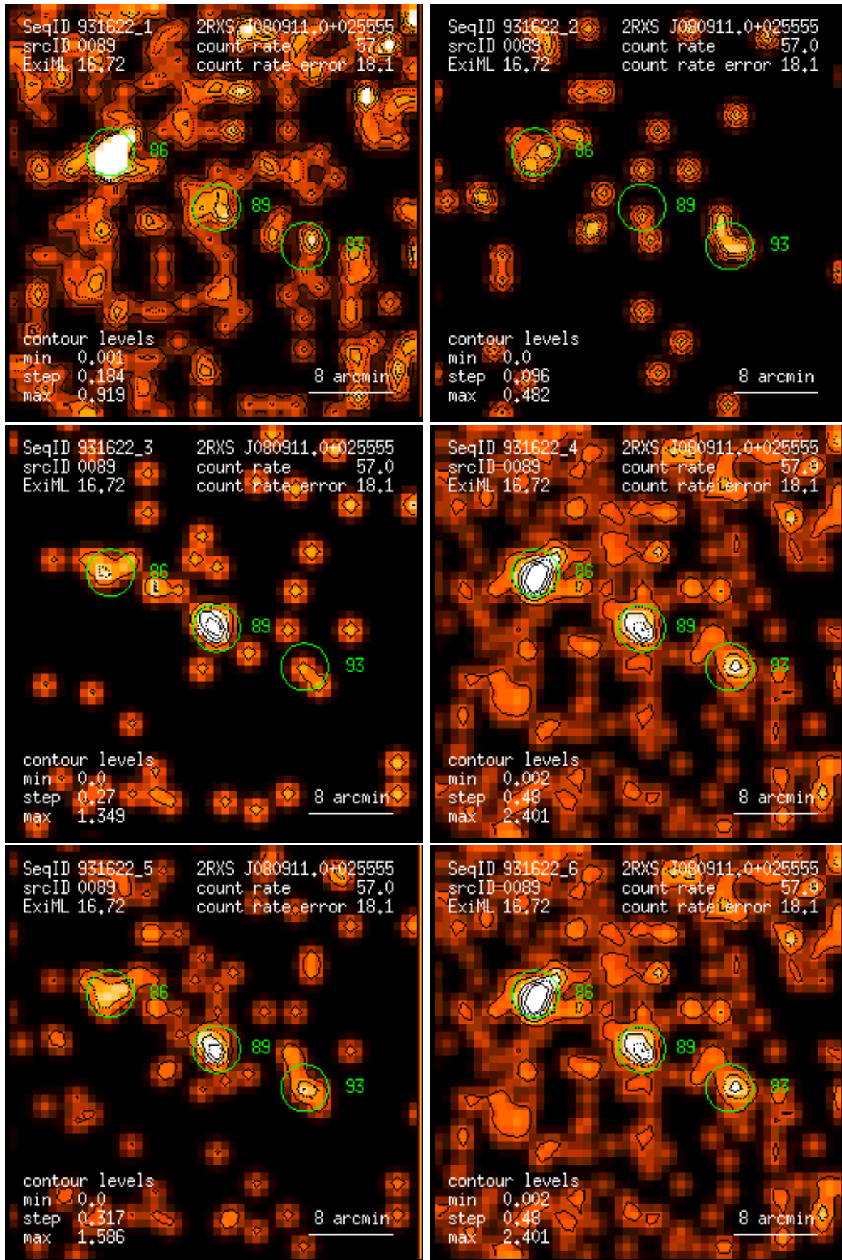
Figure 89: RASS 931622: detection 0089: band rate images, Gaussian filter: (1) PSPC channels 11 – 41, (2) 52 – 90, (3) 91 – 201, (4) 11 – 235, (5) 52 – 201, (6) 11 – 201. Broad band rates in counts/ks. Band rate contour levels in counts/ks/arcmin 2 .
