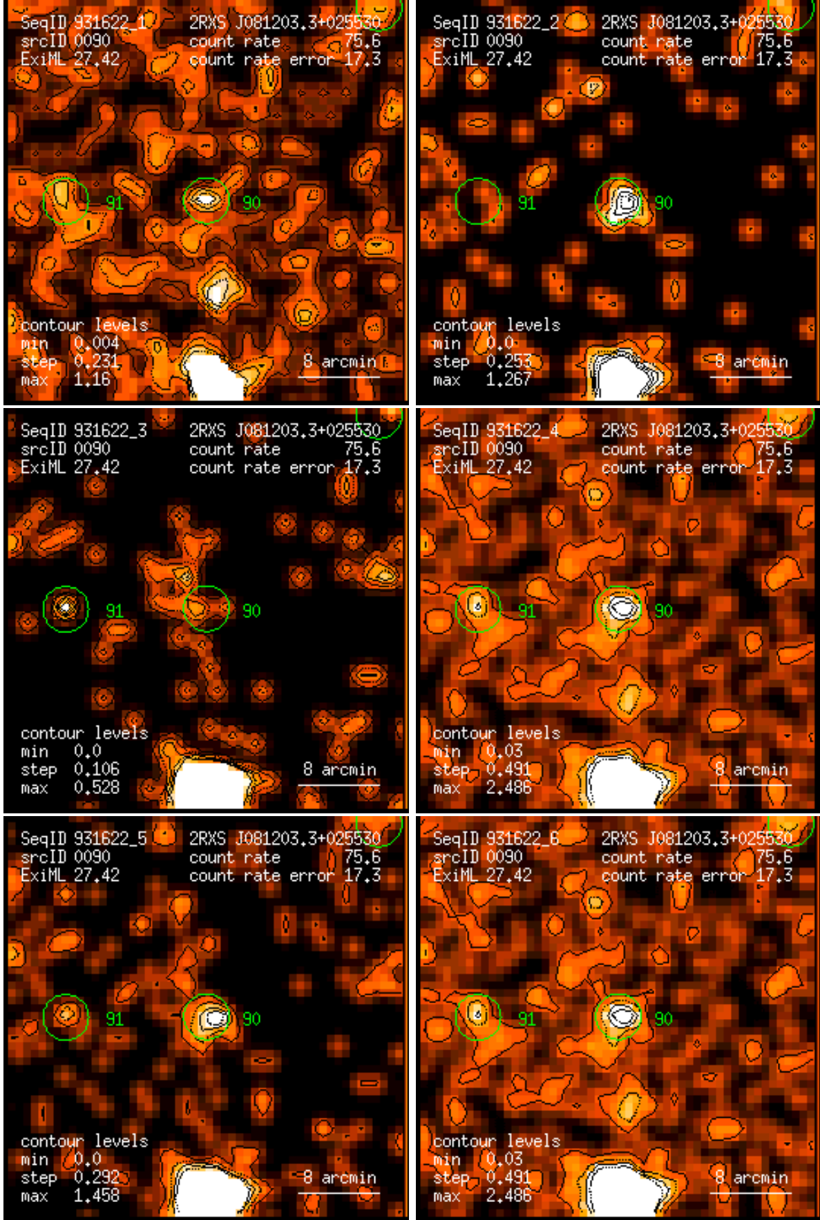
Figure 90: RASS 931622: detection 0090: band rate images, Gaussian filter: (1) PSPC channels 11 – 41, (2) 52 – 90, (3) 91 – 201, (4) 11 – 235, (5) 52 – 201, (6) 11 – 201. Broad band rates in counts/ks. Band rate contour levels in counts/ks/arcmin 2 .
