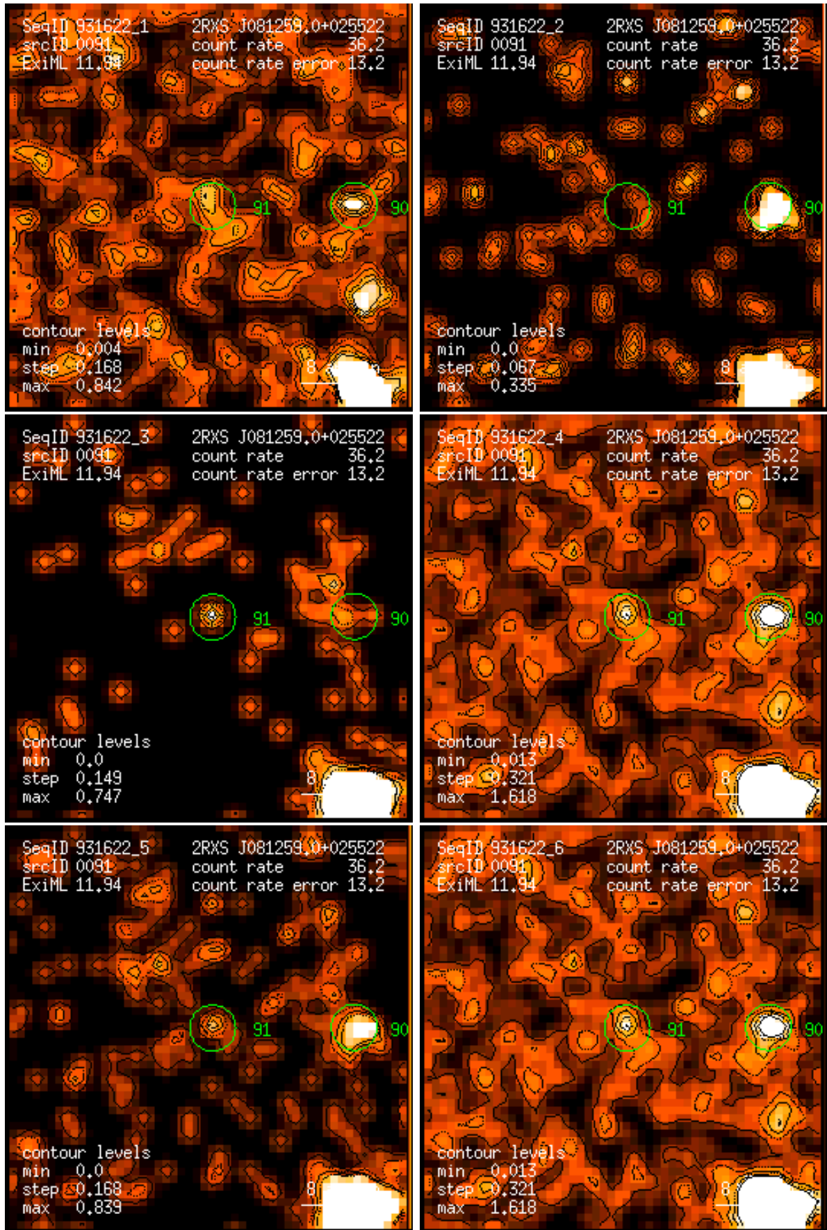
Figure 91: RASS 931622: detection 0091: band rate images, Gaussian filter: (1) PSPC channels 11 – 41, (2) 52 – 90, (3) 91 – 201, (4) 11 – 235, (5) 52 – 201, (6) 11 – 201. Broad band rates in counts/ks. Band rate contour levels in counts/ks/arcmin 2 .
