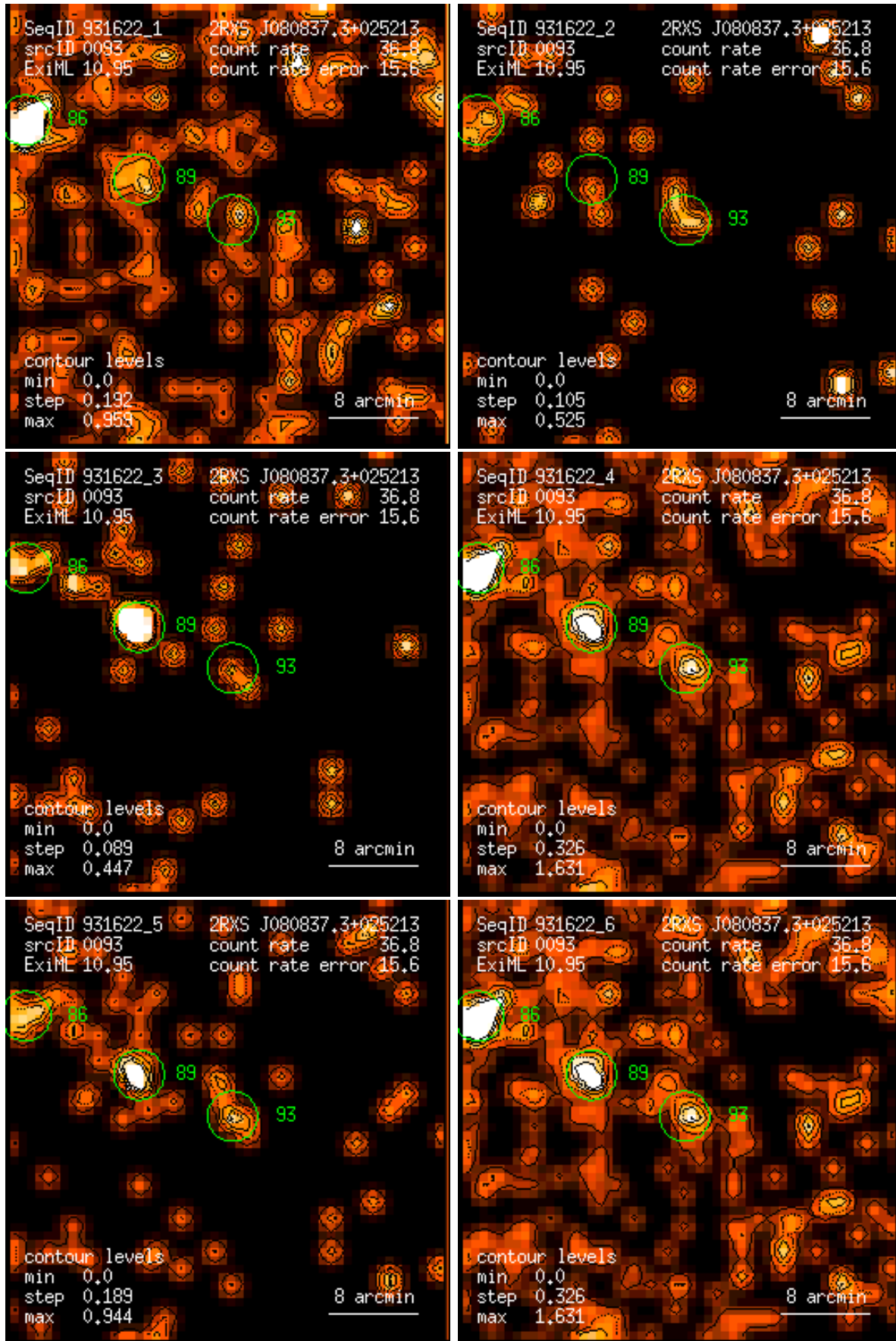
Figure 93: RASS 931622: detection 0093: band rate images, Gaussian filter: (1) PSPC channels 11 – 41, (2) 52 – 90, (3) 91 – 201, (4) 11 – 235, (5) 52 – 201, (6) 11 – 201. Broad band rates in counts/ks. Band rate contour levels in counts/ks/arcmin 2 .
