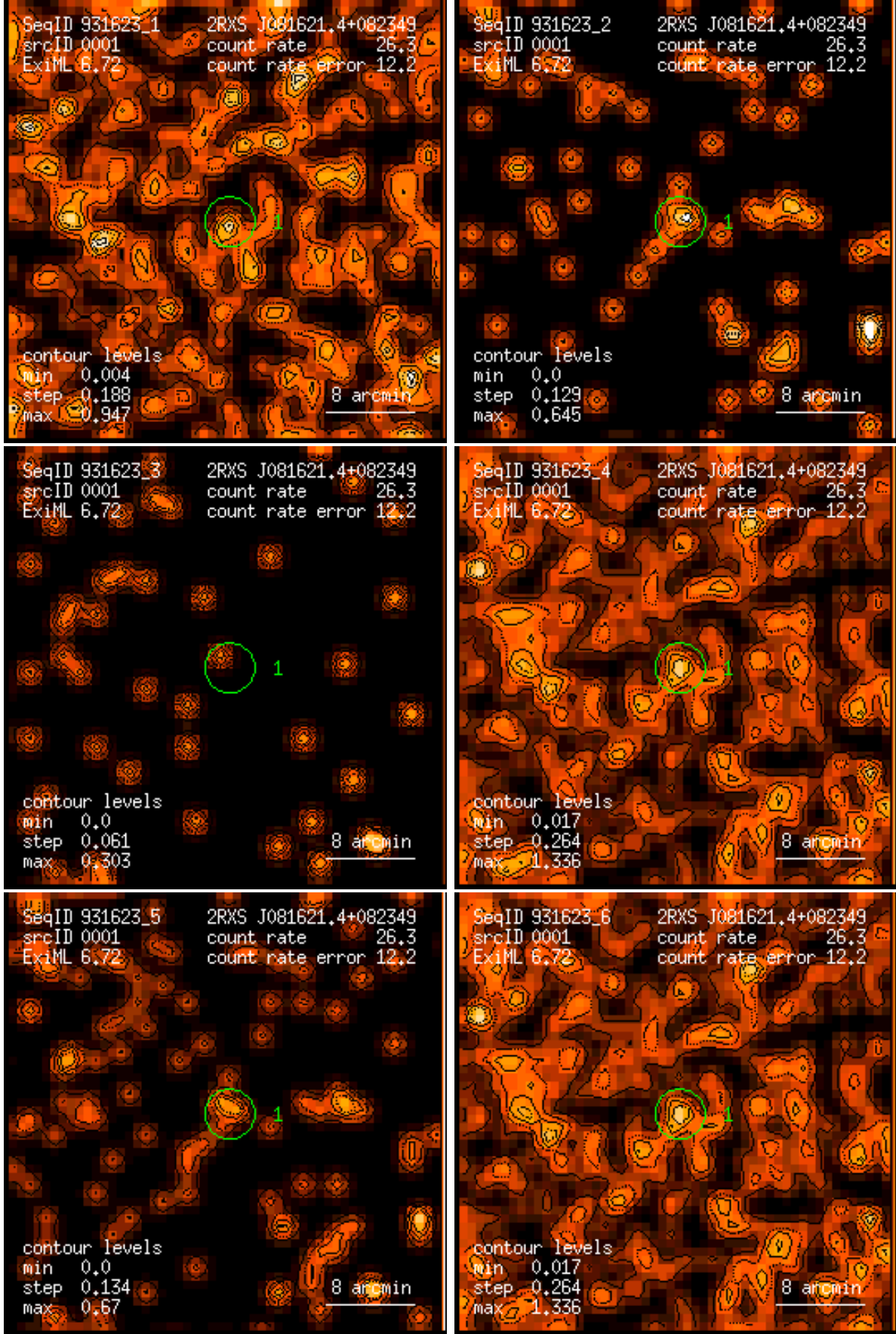
Figure 1: RASS 931623: detection 0001: band rate images, Gaussian filter: (1) PSPC channels 11 – 41, (2) 52 – 90, (3) 91 – 201, (4) 11 – 235, (5) 52 – 201, (6) 11 – 201. Broad band rates in counts/ks. Band rate contour levels in counts/ks/arcmin 2 .
