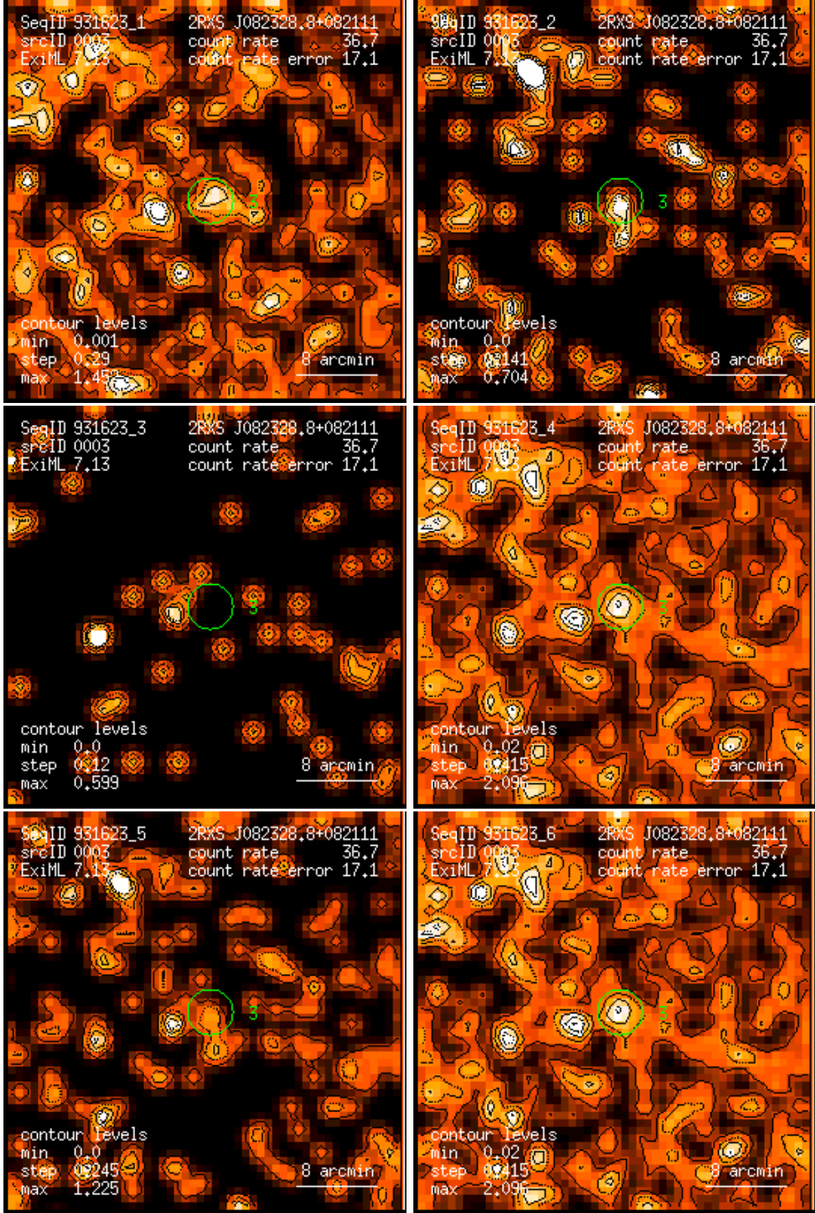
Figure 3: RASS 931623: detection 0003: band rate images, Gaussian filter: (1) PSPC channels 11 – 41, (2) 52 – 90, (3) 91 – 201, (4) 11 – 235, (5) 52 – 201, (6) 11 – 201. Broad band rates in counts/ks. Band rate contour levels in counts/ks/arcmin 2 .
