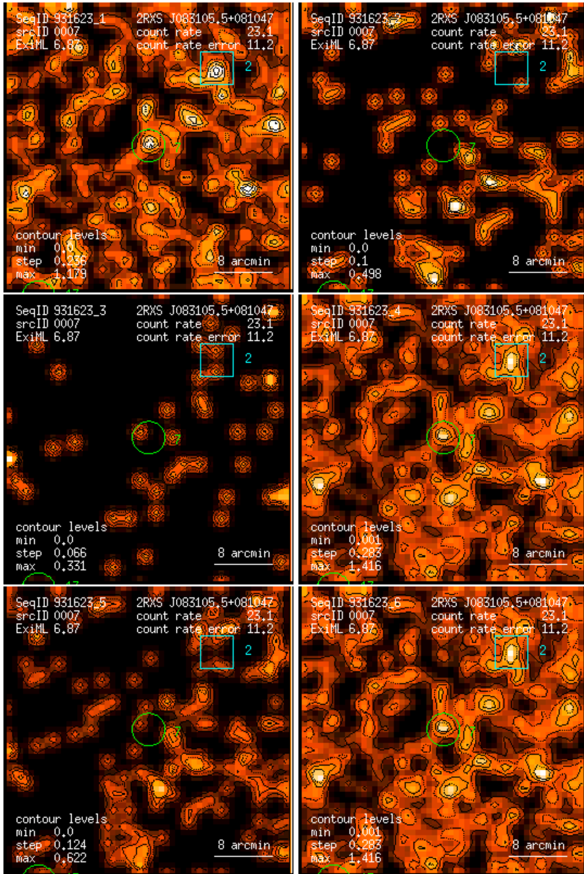
Figure 7: RASS 931623: detection 0007: band rate images, Gaussian filter: (1) PSPC channels 11 – 41, (2) 52 – 90, (3) 91 – 201, (4) 11 – 235, (5) 52 – 201, (6) 11 – 201. Broad band rates in counts/ks. Band rate contour levels in counts/ks/arcmin 2 .
