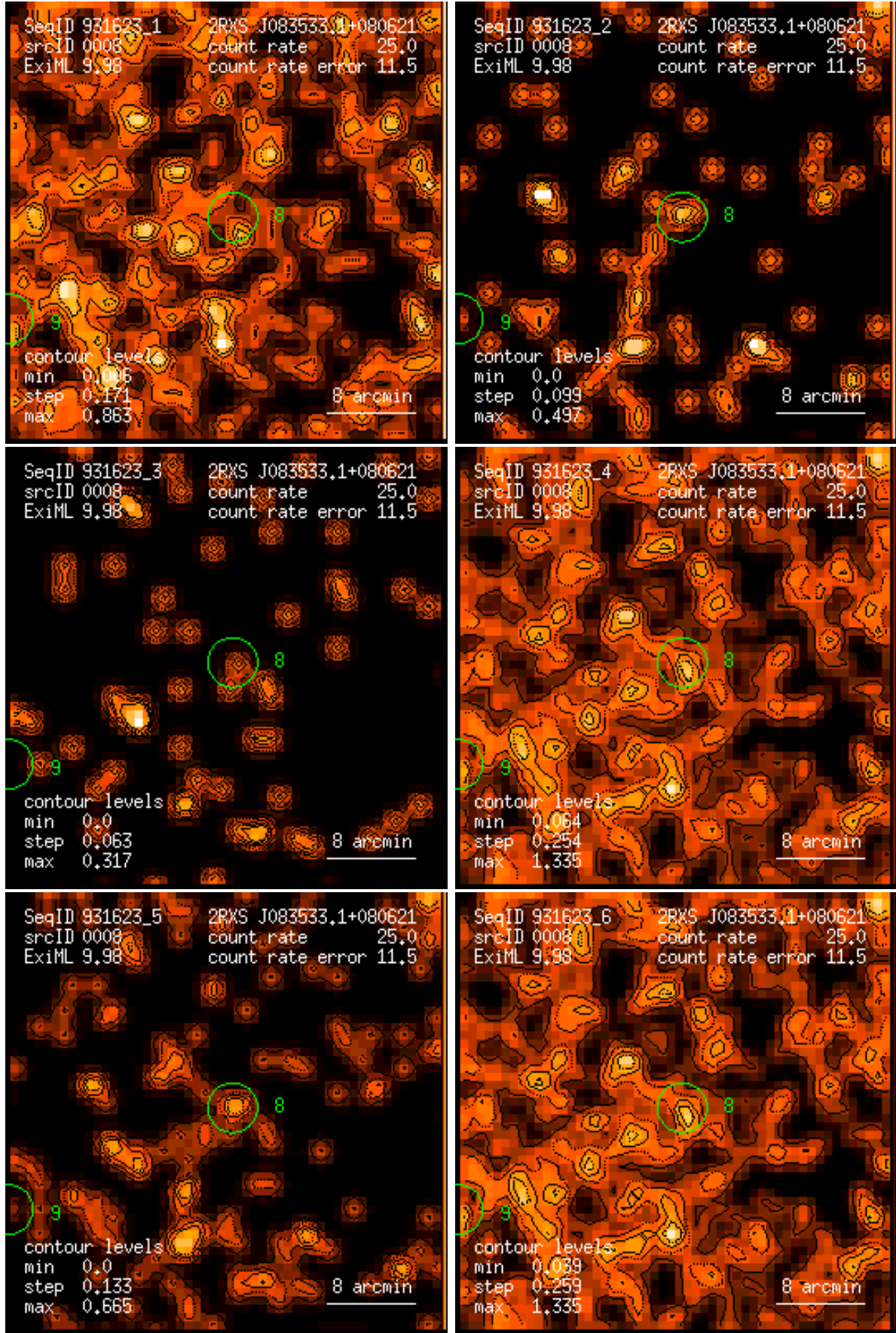
Figure 8: RASS 931623: detection 0008: band rate images, Gaussian filter: (1) PSPC channels 11 – 41, (2) 52 – 90, (3) 91 – 201, (4) 11 – 235, (5) 52 – 201, (6) 11 – 201. Broad band rates in counts/ks. Band rate contour levels in counts/ks/arcmin 2 .
