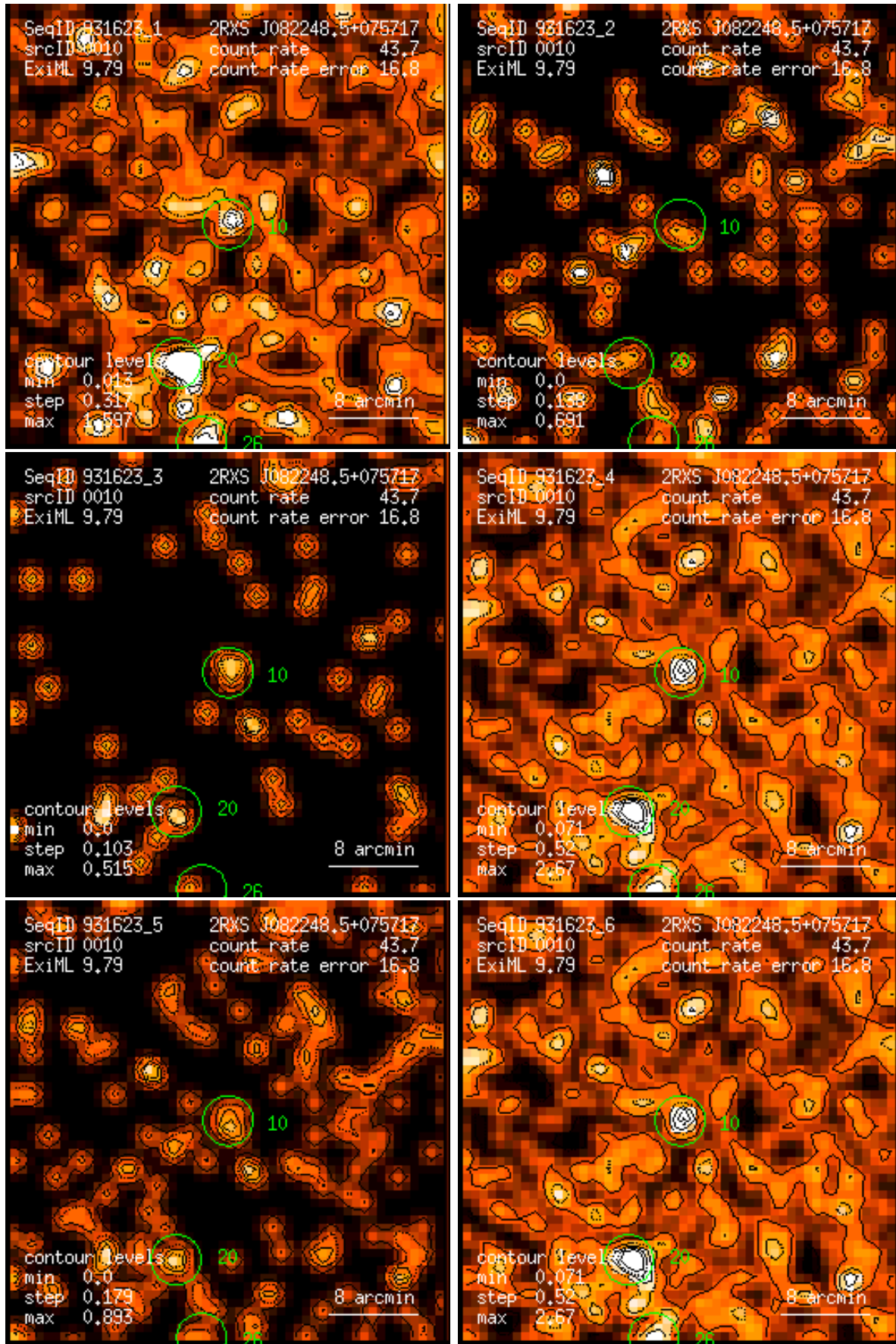
Figure 10: RASS 931623: detection 0010: band rate images, Gaussian filter: (1) PSPC channels 11 – 41, (2) 52 – 90, (3) 91 – 201, (4) 11 – 235, (5) 52 – 201, (6) 11 – 201. Broad band rates in counts/ks. Band rate contour levels in counts/ks/arcmin 2 .
