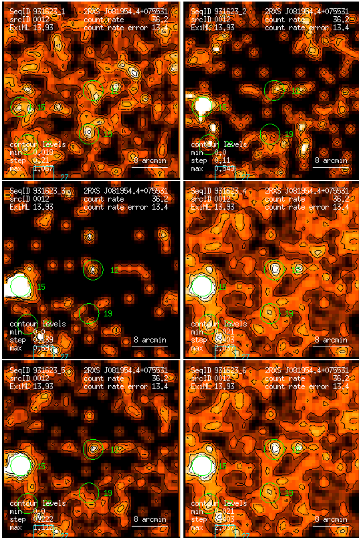
Figure 12: RASS 931623: detection 0012: band rate images, Gaussian filter: (1) PSPC channels 11 – 41, (2) 52 – 90, (3) 91 – 201, (4) 11 – 235, (5) 52 – 201, (6) 11 – 201. Broad band rates in counts/ks. Band rate contour levels in counts/ks/arcmin 2 .
