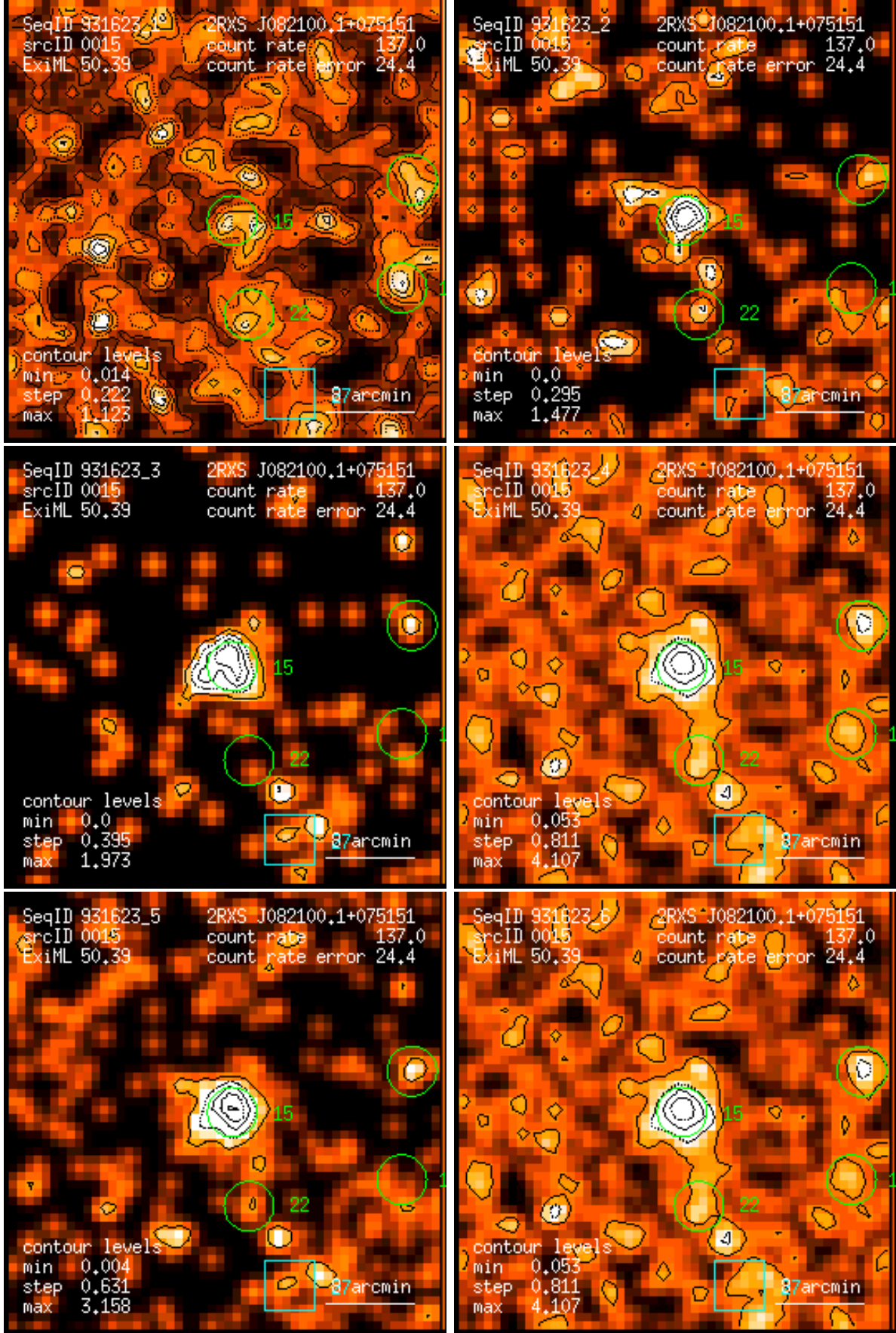
Figure 15: RASS 931623: detection 0015: band rate images, Gaussian filter: (1) PSPC channels 11 – 41, (2) 52 – 90, (3) 91 – 201, (4) 11 – 235, (5) 52 – 201, (6) 11 – 201. Broad band rates in counts/ks. Band rate contour levels in counts/ks/arcmin 2 .
