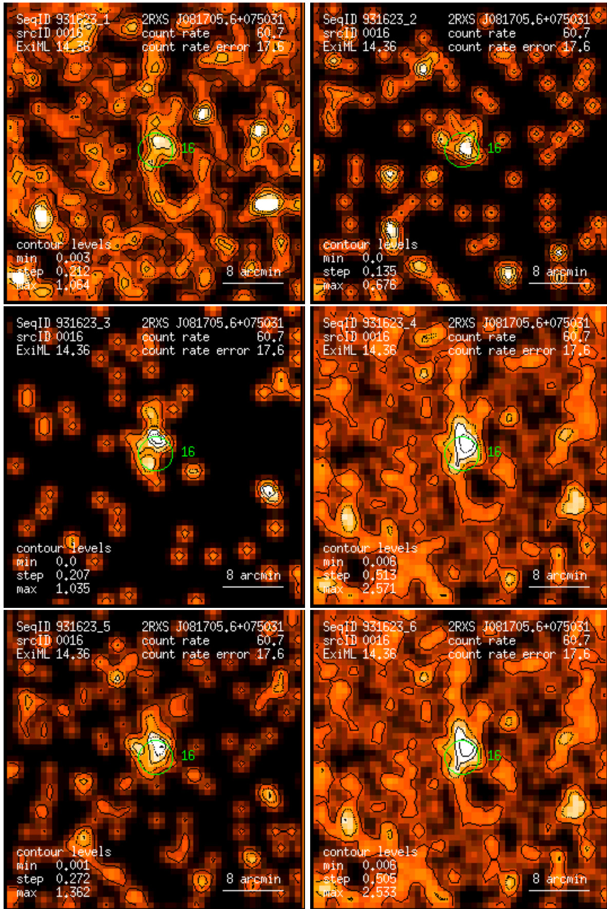
Figure 16: RASS 931623: detection 0016: band rate images, Gaussian filter: (1) PSPC channels 11 – 41, (2) 52 – 90, (3) 91 – 201, (4) 11 – 235, (5) 52 – 201, (6) 11 – 201. Broad band rates in counts/ks. Band rate contour levels in counts/ks/arcmin 2 .
