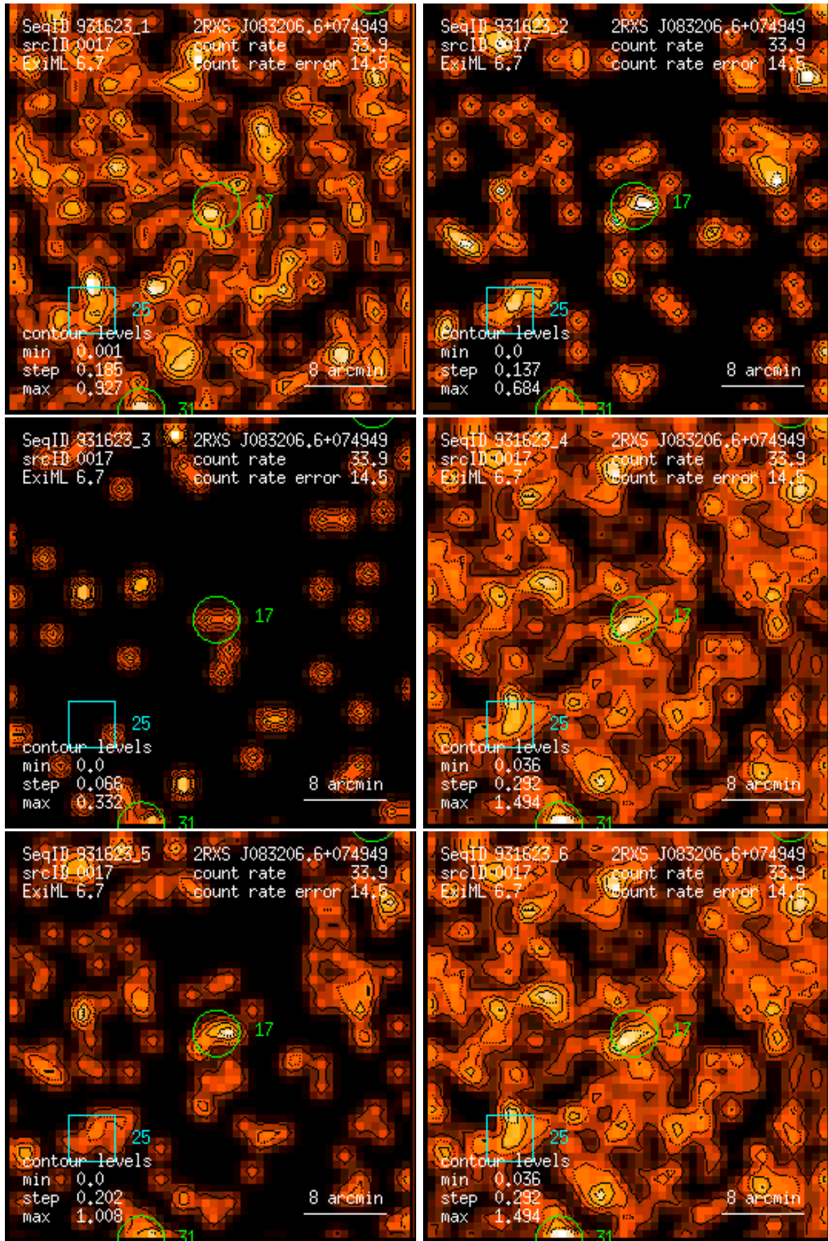
Figure 17: RASS 931623: detection 0017: band rate images, Gaussian filter: (1) PSPC channels 11 – 41, (2) 52 – 90, (3) 91 – 201, (4) 11 – 235, (5) 52 – 201, (6) 11 – 201. Broad band rates in counts/ks. Band rate contour levels in counts/ks/arcmin 2 .
