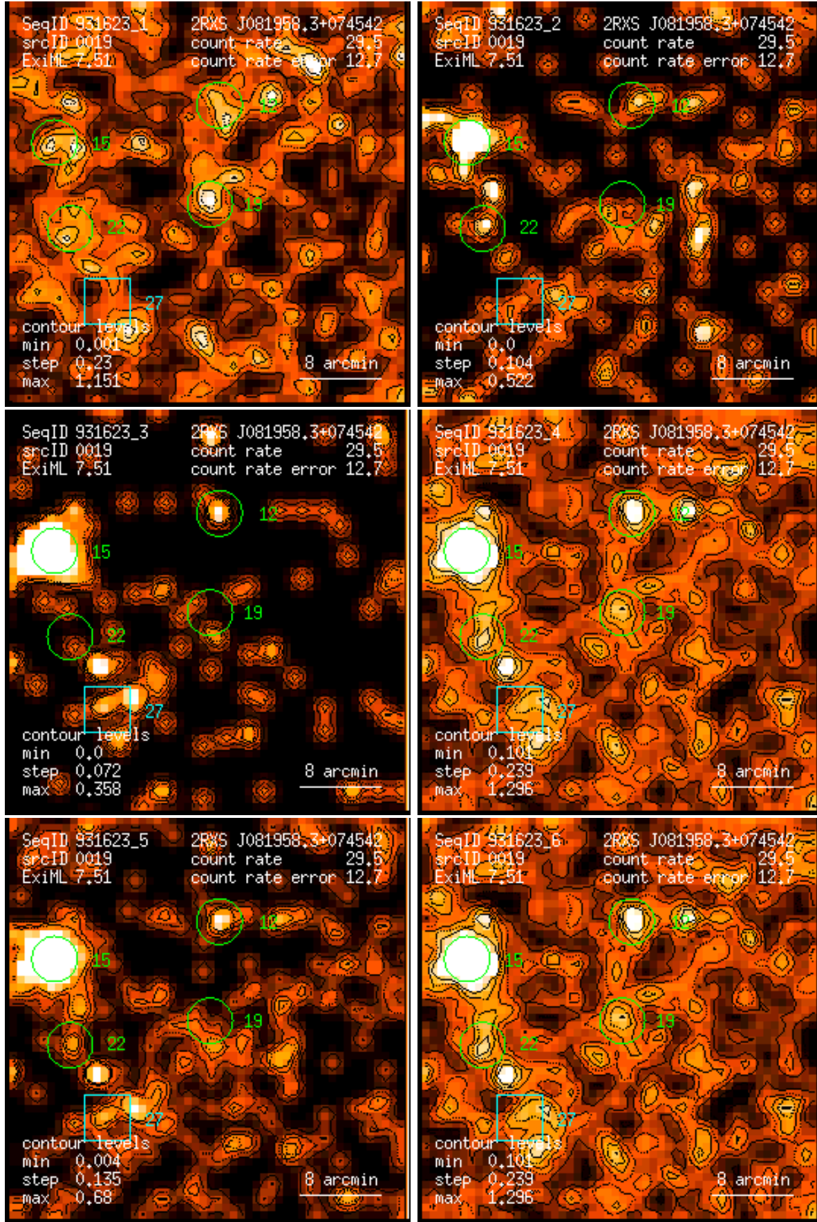
Figure 19: RASS 931623: detection 0019: band rate images, Gaussian filter: (1) PSPC channels 11 – 41, (2) 52 – 90, (3) 91 – 201, (4) 11 – 235, (5) 52 – 201, (6) 11 – 201. Broad band rates in counts/ks. Band rate contour levels in counts/ks/arcmin 2 .
