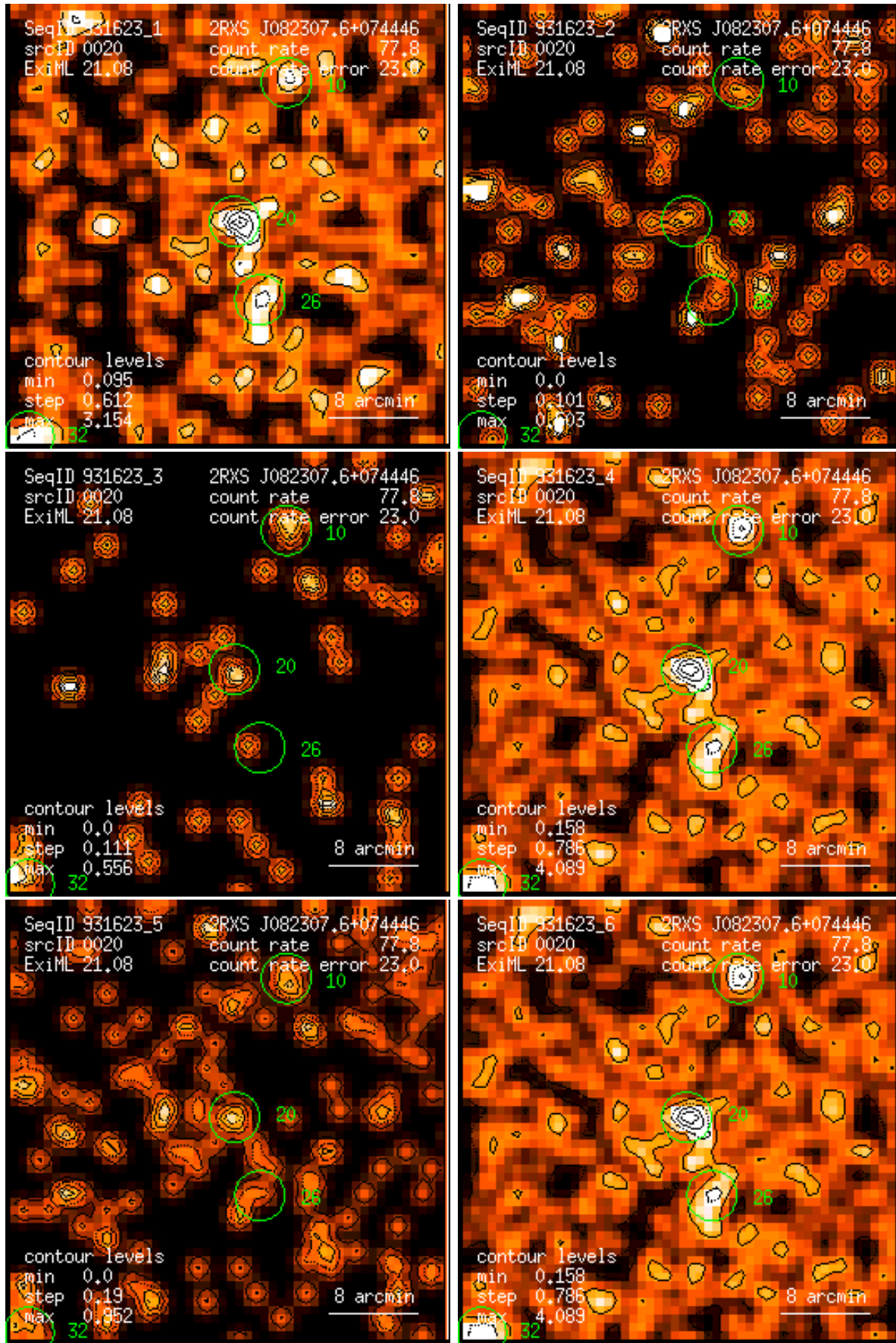
Figure 20: RASS 931623: detection 0020: band rate images, Gaussian filter: (1) PSPC channels 11 – 41, (2) 52 – 90, (3) 91 – 201, (4) 11 – 235, (5) 52 – 201, (6) 11 – 201. Broad band rates in counts/ks. Band rate contour levels in counts/ks/arcmin 2 .
