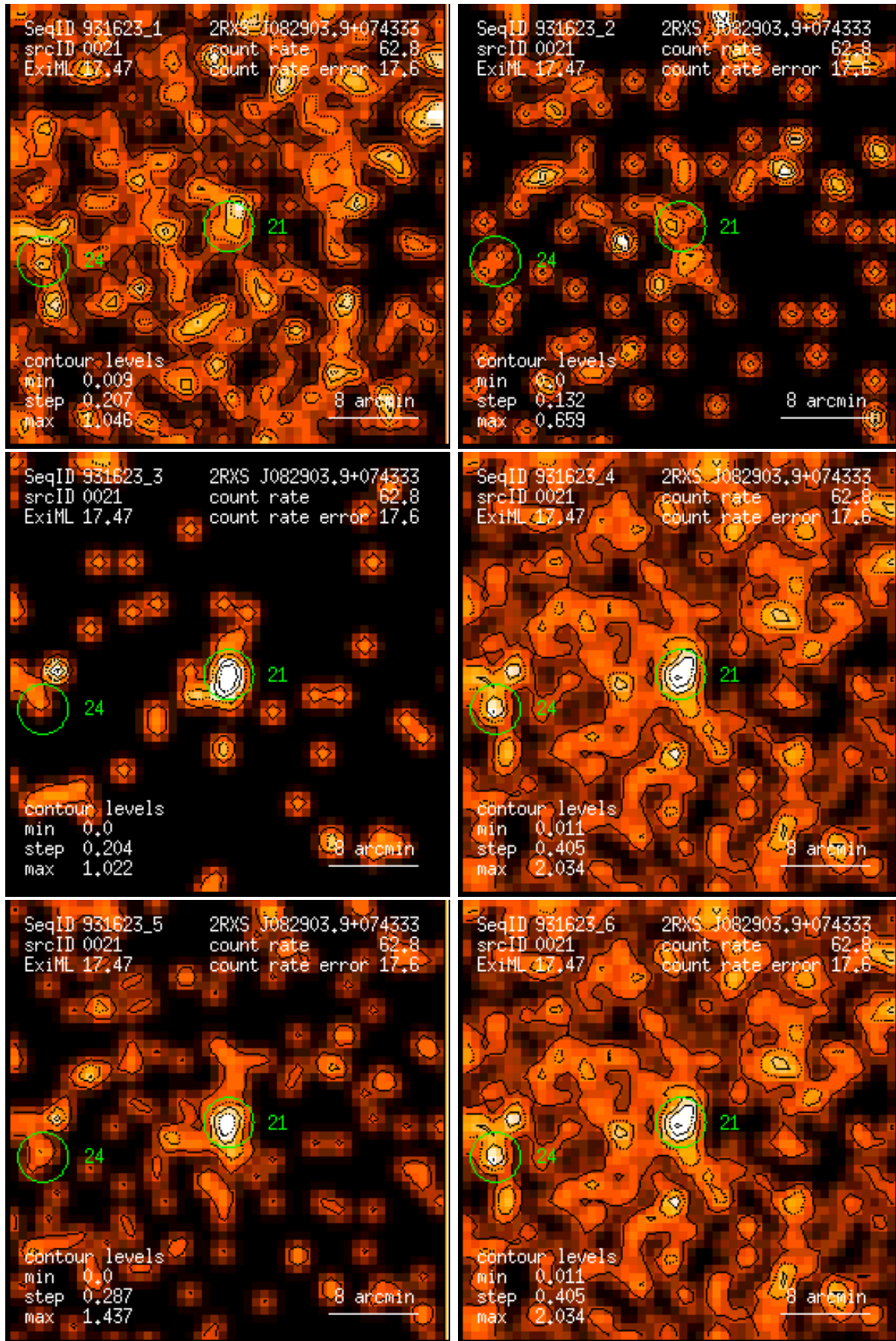
Figure 21: RASS 931623: detection 0021: band rate images, Gaussian filter: (1) PSPC channels 11 – 41, (2) 52 – 90, (3) 91 – 201, (4) 11 – 235, (5) 52 – 201, (6) 11 – 201. Broad band rates in counts/ks. Band rate contour levels in counts/ks/arcmin 2 .
