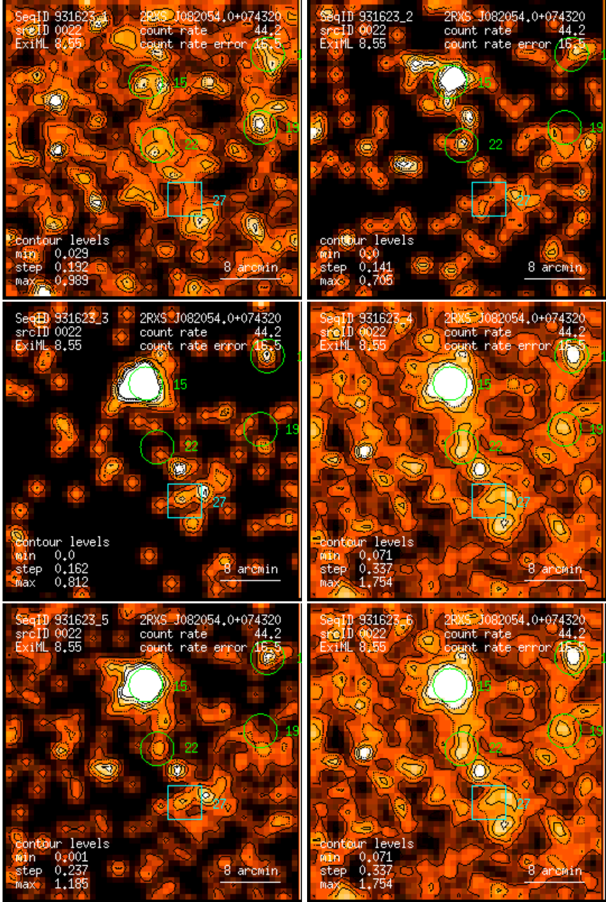
Figure 22: RASS 931623: detection 0022: band rate images, Gaussian filter: (1) PSPC channels 11 – 41, (2) 52 – 90, (3) 91 – 201, (4) 11 – 235, (5) 52 – 201, (6) 11 – 201. Broad band rates in counts/ks. Band rate contour levels in counts/ks/arcmin 2 .
