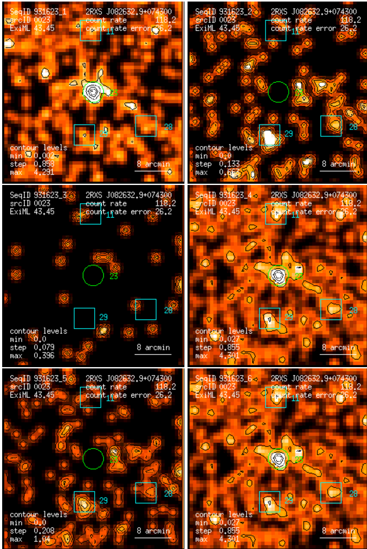
Figure 23: RASS 931623: detection 0023: band rate images, Gaussian filter: (1) PSPC channels 11 – 41, (2) 52 – 90, (3) 91 – 201, (4) 11 – 235, (5) 52 – 201, (6) 11 – 201. Broad band rates in counts/ks. Band rate contour levels in counts/ks/arcmin 2 .
