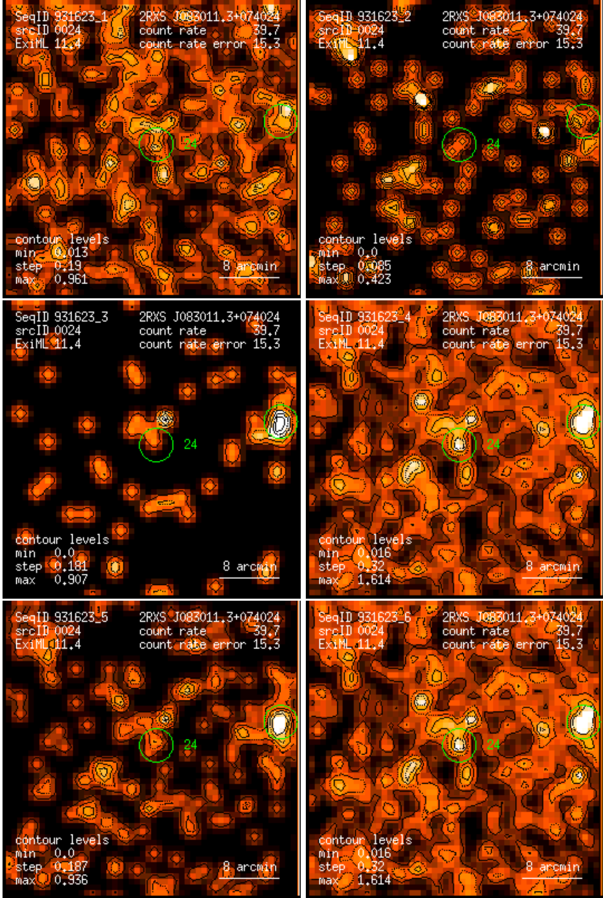
Figure 24: RASS 931623: detection 0024: band rate images, Gaussian filter: (1) PSPC channels 11 – 41, (2) 52 – 90, (3) 91 – 201, (4) 11 – 235, (5) 52 – 201, (6) 11 – 201. Broad band rates in counts/ks. Band rate contour levels in counts/ks/arcmin 2 .
