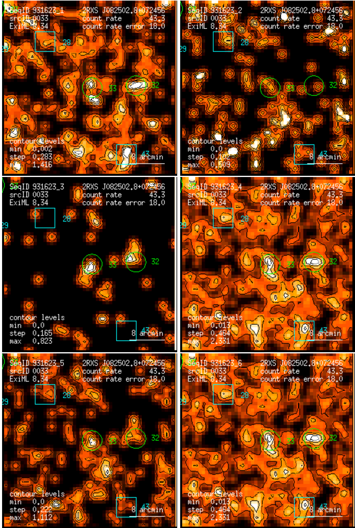
Figure 33: RASS 931623: detection 0033: band rate images, Gaussian filter: (1) PSPC channels 11 – 41, (2) 52 – 90, (3) 91 – 201, (4) 11 – 235, (5) 52 – 201, (6) 11 – 201. Broad band rates in counts/ks. Band rate contour levels in counts/ks/arcmin 2 .
