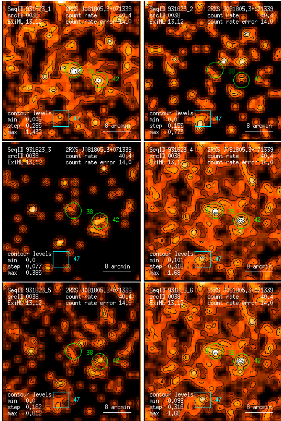
Figure 38: RASS 931623: detection 0038: band rate images, Gaussian filter: (1) PSPC channels 11 – 41, (2) 52 – 90, (3) 91 – 201, (4) 11 – 235, (5) 52 – 201, (6) 11 – 201. Broad band rates in counts/ks. Band rate contour levels in counts/ks/arcmin 2 .
