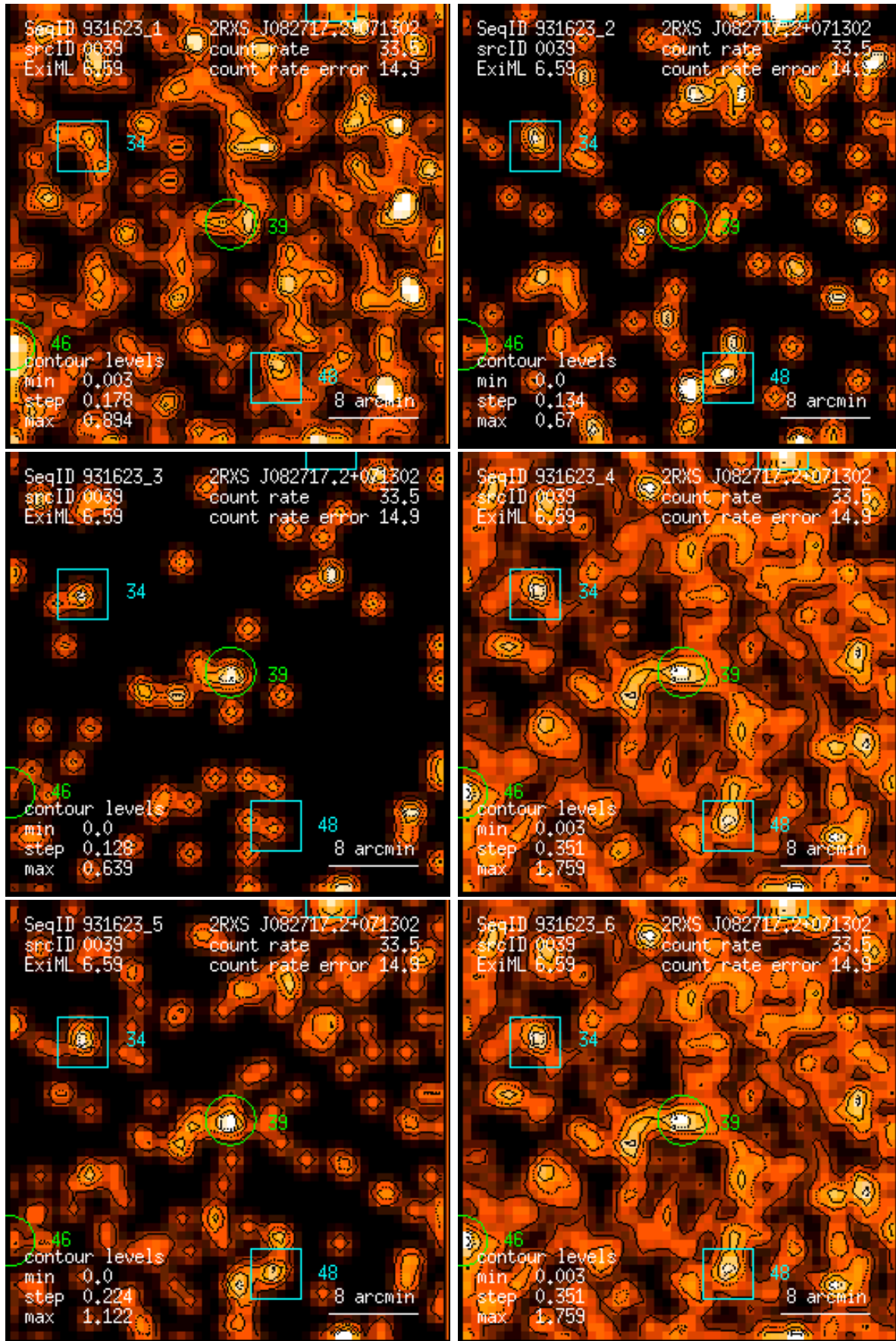
Figure 39: RASS 931623: detection 0039: band rate images, Gaussian filter: (1) PSPC channels 11 – 41, (2) 52 – 90, (3) 91 – 201, (4) 11 – 235, (5) 52 – 201, (6) 11 – 201. Broad band rates in counts/ks. Band rate contour levels in counts/ks/arcmin 2 .
