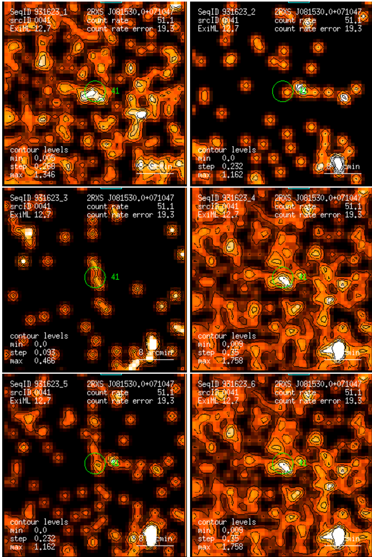
Figure 41: RASS 931623: detection 0041: band rate images, Gaussian filter: (1) PSPC channels 11 – 41, (2) 52 – 90, (3) 91 – 201, (4) 11 – 235, (5) 52 – 201, (6) 11 – 201. Broad band rates in counts/ks. Band rate contour levels in counts/ks/arcmin 2 .
