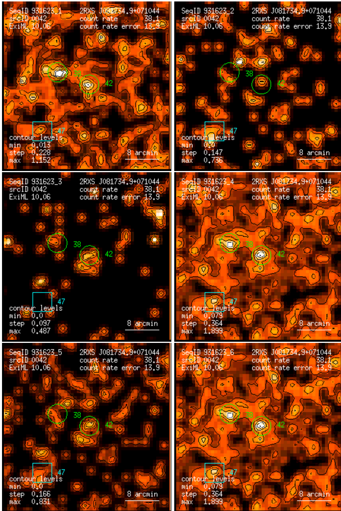
Figure 42: RASS 931623: detection 0042: band rate images, Gaussian filter: (1) PSPC channels 11 – 41, (2) 52 – 90, (3) 91 – 201, (4) 11 – 235, (5) 52 – 201, (6) 11 – 201. Broad band rates in counts/ks. Band rate contour levels in counts/ks/arcmin 2 .
