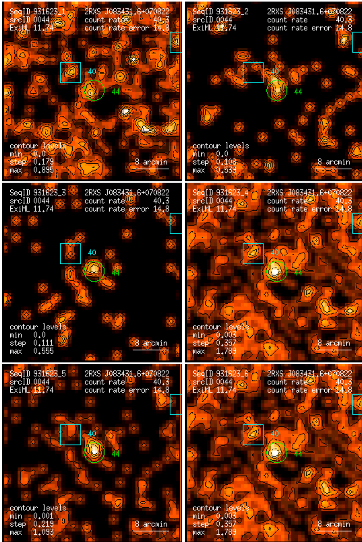
Figure 44: RASS 931623: detection 0044: band rate images, Gaussian filter: (1) PSPC channels 11 – 41, (2) 52 – 90, (3) 91 – 201, (4) 11 – 235, (5) 52 – 201, (6) 11 – 201. Broad band rates in counts/ks. Band rate contour levels in counts/ks/arcmin 2 .
