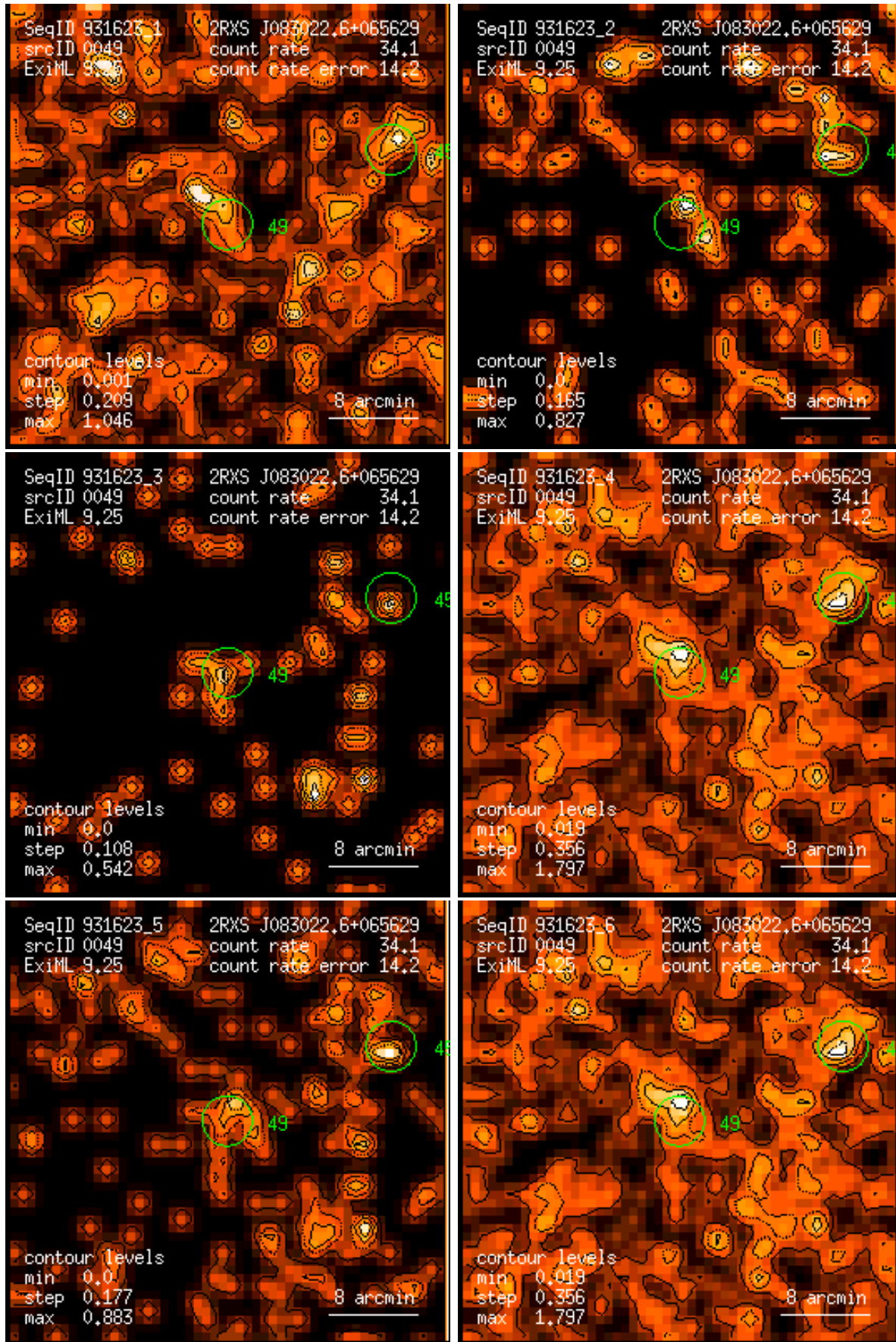
Figure 49: RASS 931623: detection 0049: band rate images, Gaussian filter: (1) PSPC channels 11 – 41, (2) 52 – 90, (3) 91 – 201, (4) 11 – 235, (5) 52 – 201, (6) 11 – 201. Broad band rates in counts/ks. Band rate contour levels in counts/ks/arcmin 2 .
