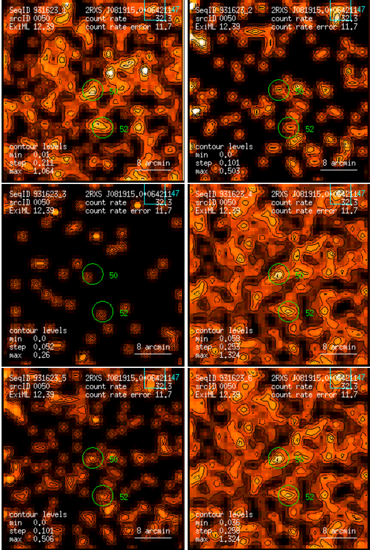
Figure 50: RASS 931623: detection 0050: band rate images, Gaussian filter: (1) PSPC channels 11 – 41, (2) 52 – 90, (3) 91 – 201, (4) 11 – 235, (5) 52 – 201, (6) 11 – 201. Broad band rates in counts/ks. Band rate contour levels in counts/ks/arcmin 2 .
