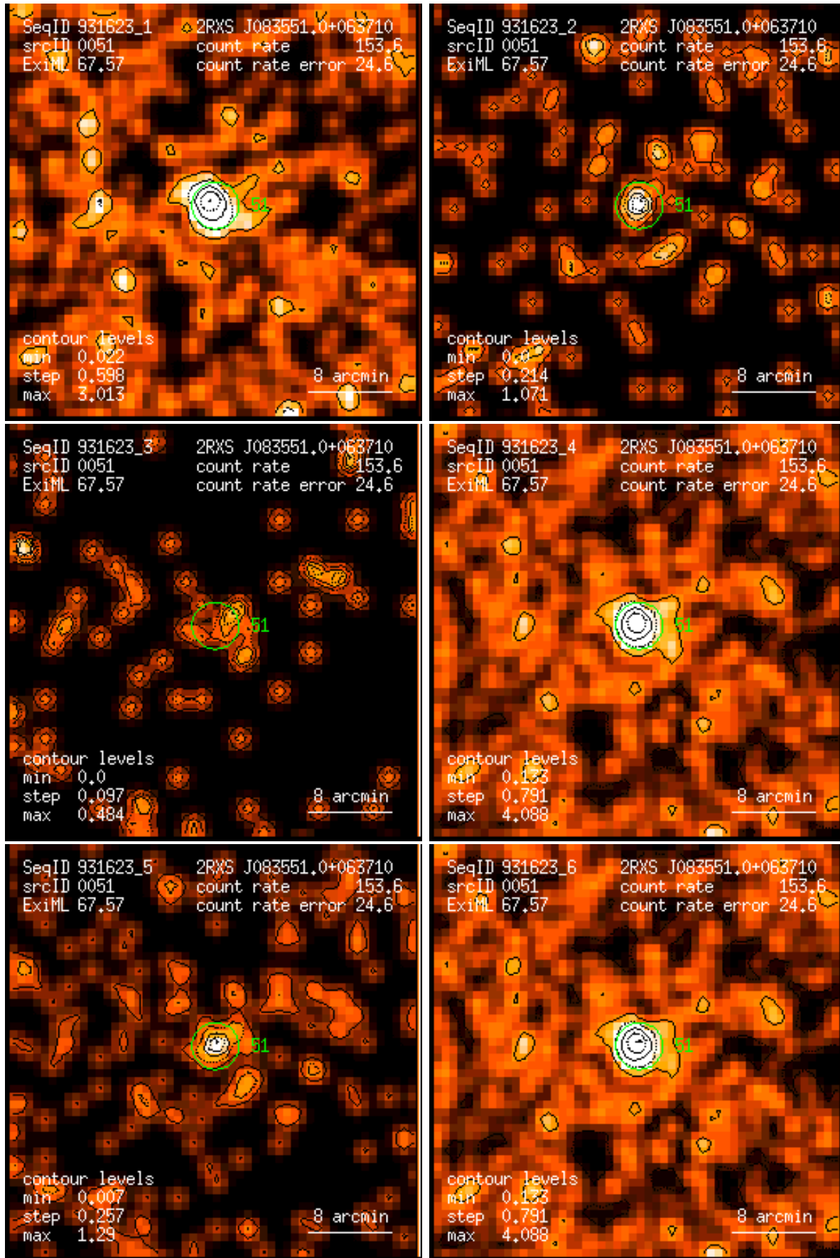
Figure 51: RASS 931623: detection 0051: band rate images, Gaussian filter: (1) PSPC channels 11 – 41, (2) 52 – 90, (3) 91 – 201, (4) 11 – 235, (5) 52 – 201, (6) 11 – 201. Broad band rates in counts/ks. Band rate contour levels in counts/ks/arcmin 2 .
