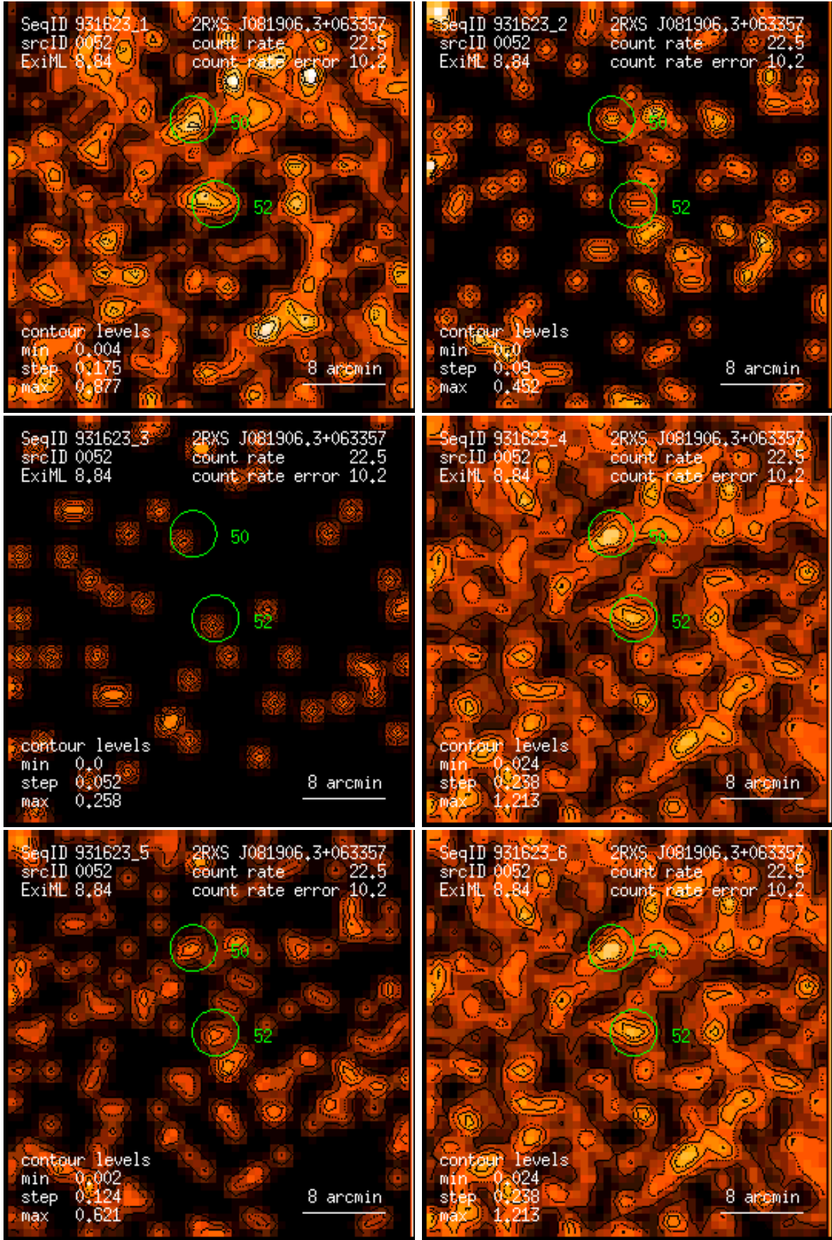
Figure 52: RASS 931623: detection 0052: band rate images, Gaussian filter: (1) PSPC channels 11 – 41, (2) 52 – 90, (3) 91 – 201, (4) 11 – 235, (5) 52 – 201, (6) 11 – 201. Broad band rates in counts/ks. Band rate contour levels in counts/ks/arcmin 2 .
