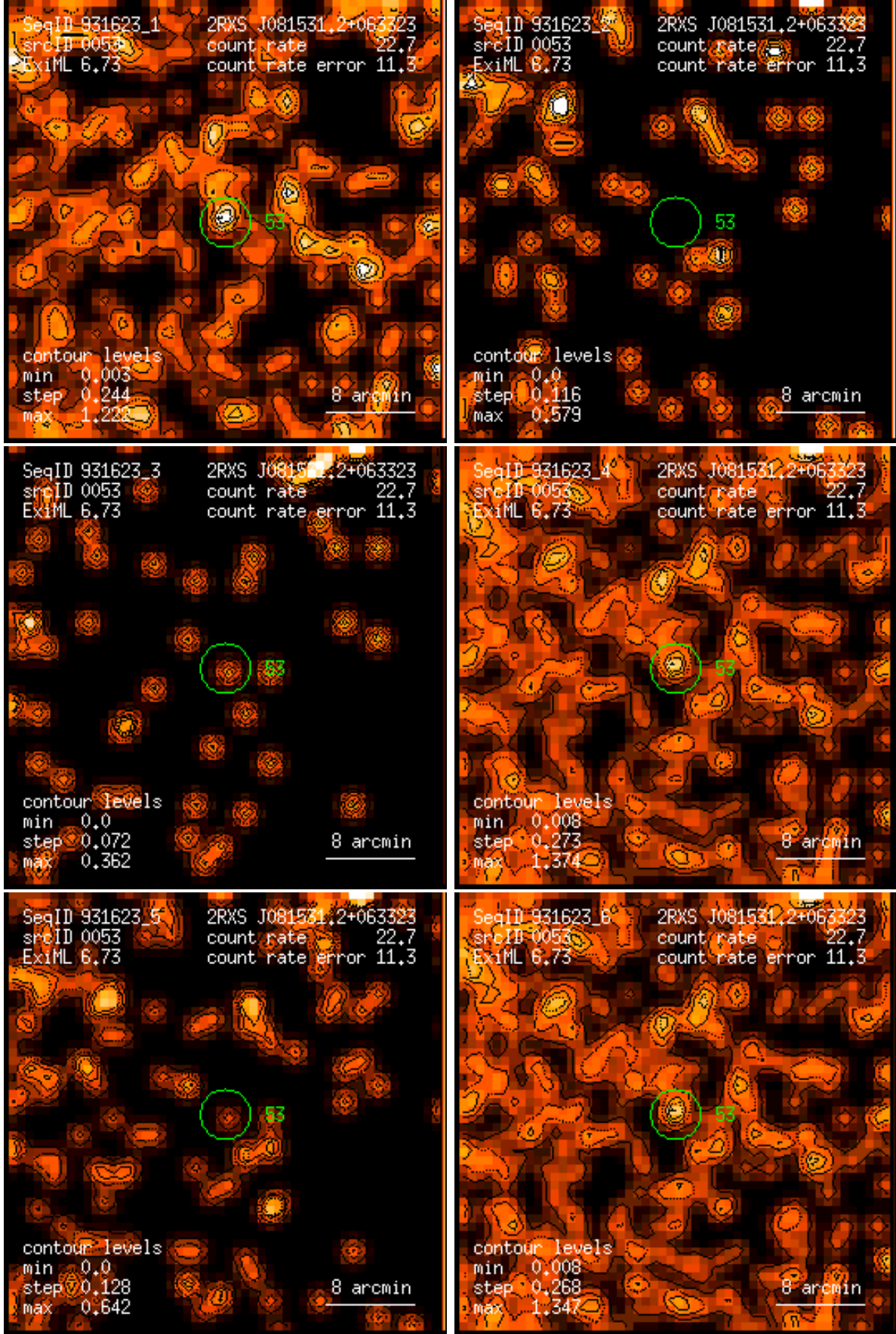
Figure 53: RASS 931623: detection 0053: band rate images, Gaussian filter: (1) PSPC channels 11 – 41, (2) 52 – 90, (3) 91 – 201, (4) 11 – 235, (5) 52 – 201, (6) 11 – 201. Broad band rates in counts/ks. Band rate contour levels in counts/ks/arcmin 2 .
