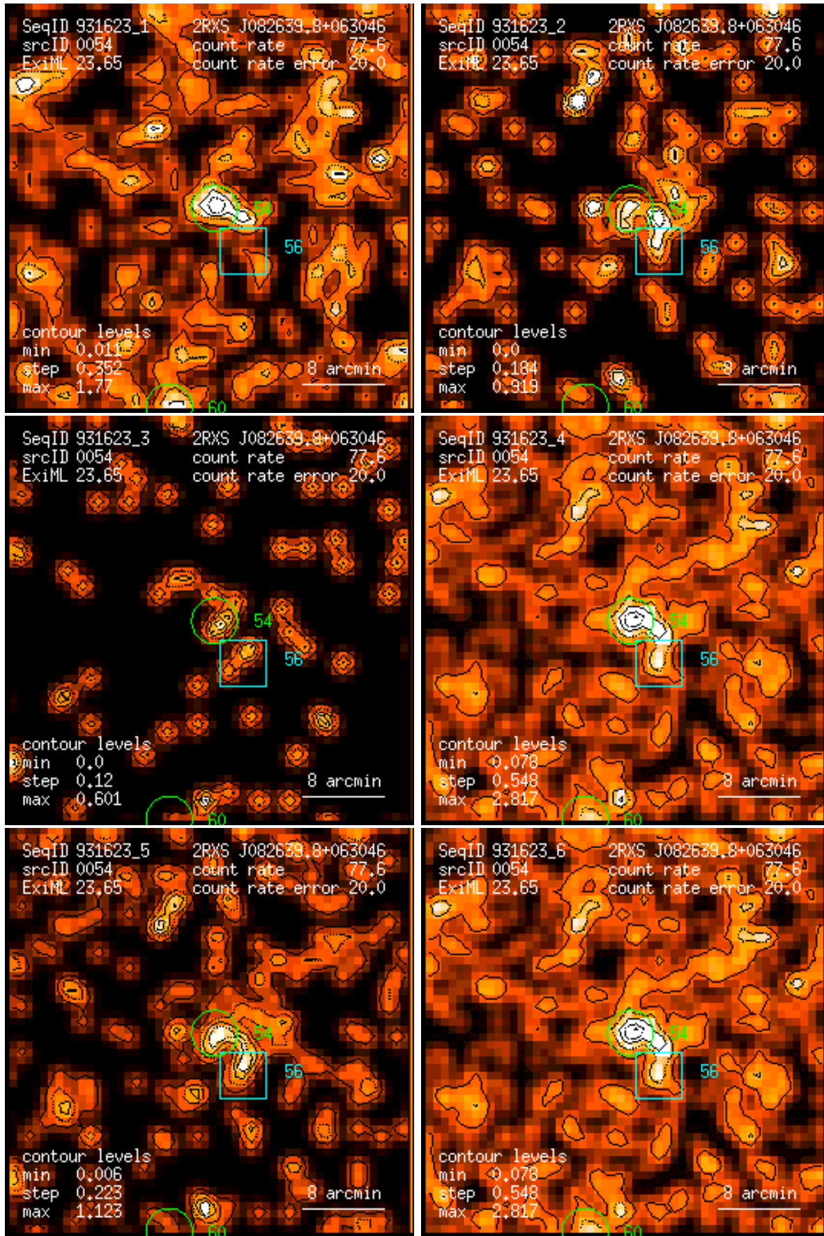
Figure 54: RASS 931623: detection 0054: band rate images, Gaussian filter: (1) PSPC channels 11 – 41, (2) 52 – 90, (3) 91 – 201, (4) 11 – 235, (5) 52 – 201, (6) 11 – 201. Broad band rates in counts/ks. Band rate contour levels in counts/ks/arcmin 2 .
