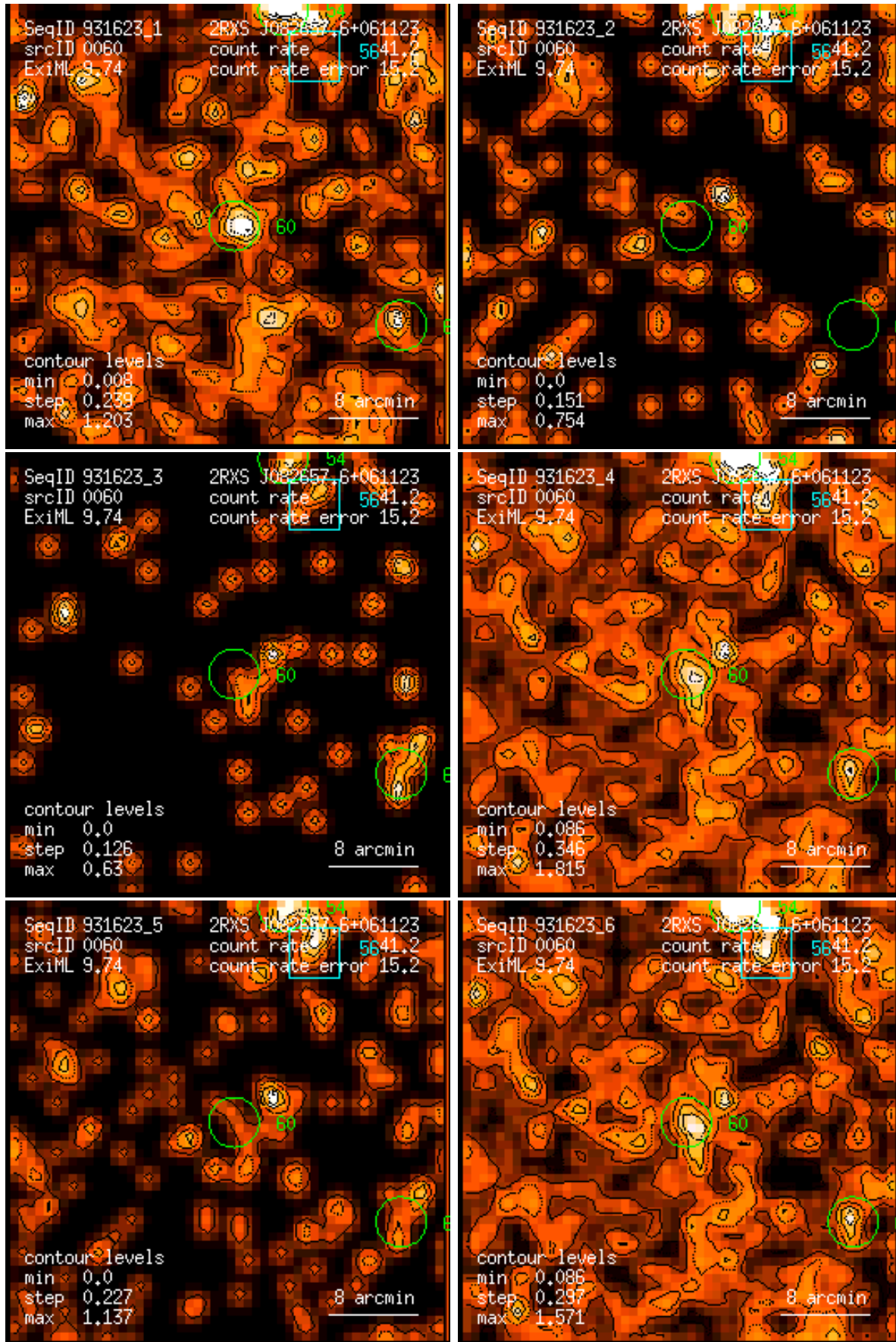
Figure 60: RASS 931623: detection 0060: band rate images, Gaussian filter: (1) PSPC channels 11 – 41, (2) 52 – 90, (3) 91 – 201, (4) 11 – 235, (5) 52 – 201, (6) 11 – 201. Broad band rates in counts/ks. Band rate contour levels in counts/ks/arcmin 2 .
