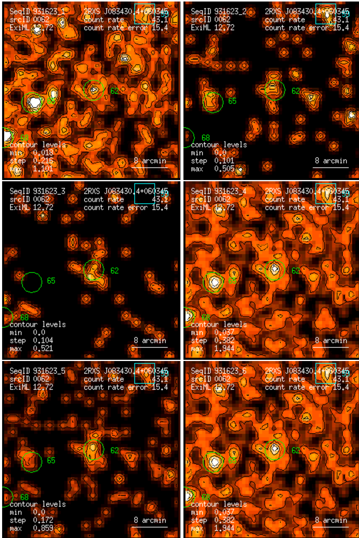
Figure 62: RASS 931623: detection 0062: band rate images, Gaussian filter: (1) PSPC channels 11 – 41, (2) 52 – 90, (3) 91 – 201, (4) 11 – 235, (5) 52 – 201, (6) 11 – 201. Broad band rates in counts/ks. Band rate contour levels in counts/ks/arcmin 2 .
