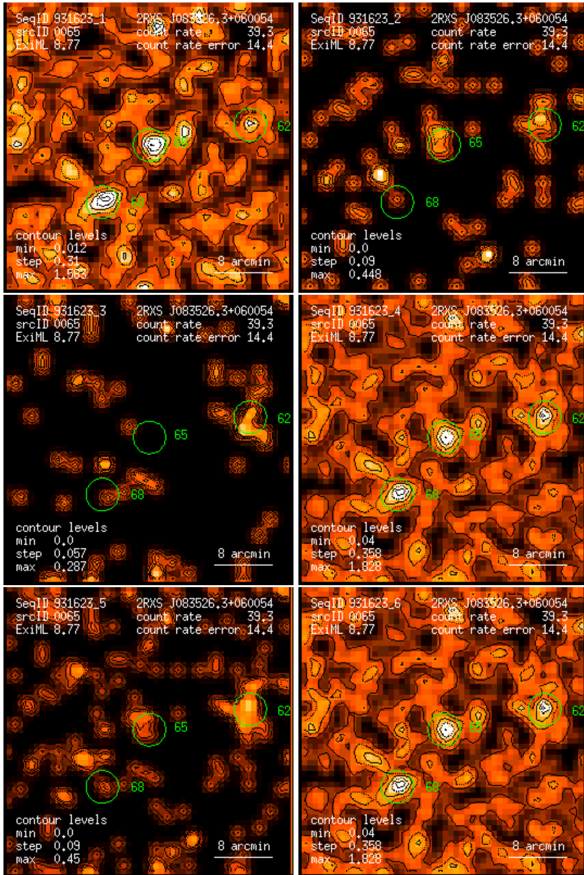
Figure 65: RASS 931623: detection 0065: band rate images, Gaussian filter: (1) PSPC channels 11 – 41, (2) 52 – 90, (3) 91 – 201, (4) 11 – 235, (5) 52 – 201, (6) 11 – 201. Broad band rates in counts/ks. Band rate contour levels in counts/ks/arcmin 2 .
