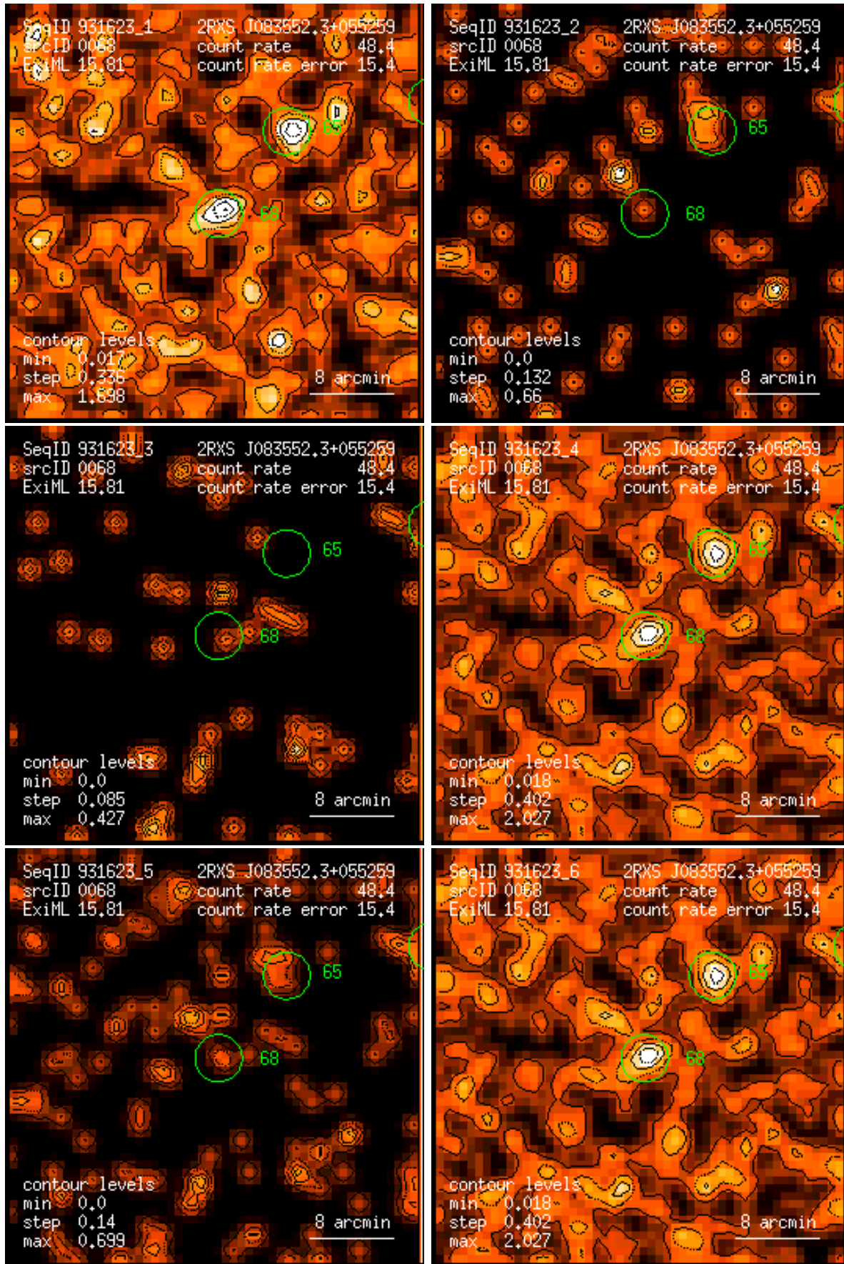
Figure 68: RASS 931623: detection 0068: band rate images, Gaussian filter: (1) PSPC channels 11 – 41, (2) 52 – 90, (3) 91 – 201, (4) 11 – 235, (5) 52 – 201, (6) 11 – 201. Broad band rates in counts/ks. Band rate contour levels in counts/ks/arcmin 2 .
