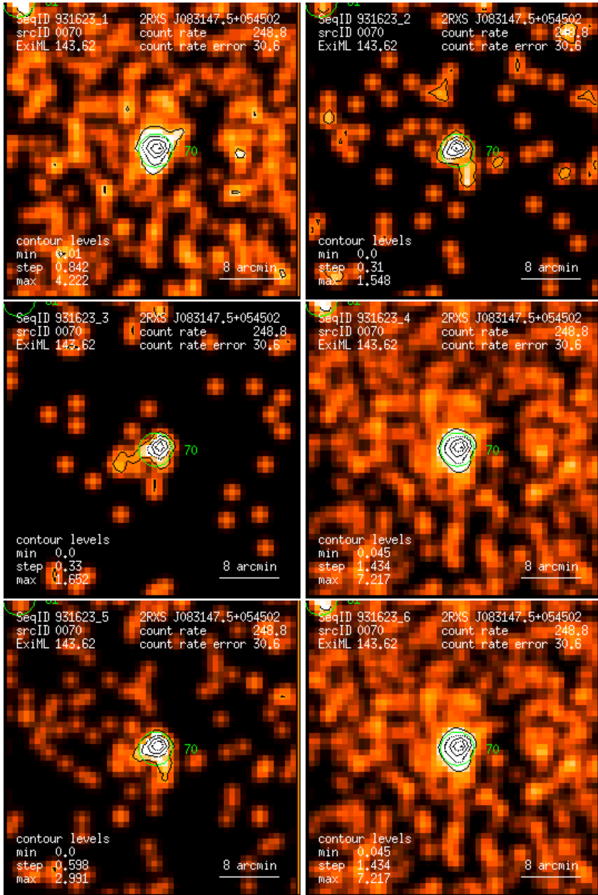
Figure 70: RASS 931623: detection 0070: band rate images, Gaussian filter: (1) PSPC channels 11 – 41, (2) 52 – 90, (3) 91 – 201, (4) 11 – 235, (5) 52 – 201, (6) 11 – 201. Broad band rates in counts/ks. Band rate contour levels in counts/ks/arcmin 2 .
