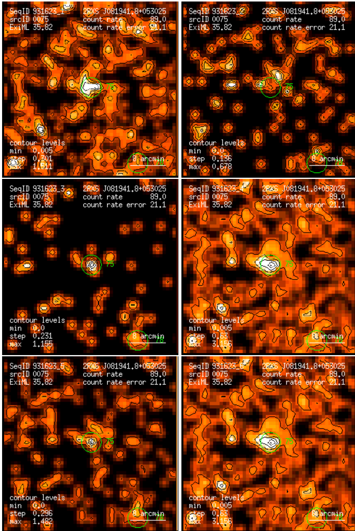
Figure 75: RASS 931623: detection 0075: band rate images, Gaussian filter: (1) PSPC channels 11 – 41, (2) 52 – 90, (3) 91 – 201, (4) 11 – 235, (5) 52 – 201, (6) 11 – 201. Broad band rates in counts/ks. Band rate contour levels in counts/ks/arcmin 2 .
