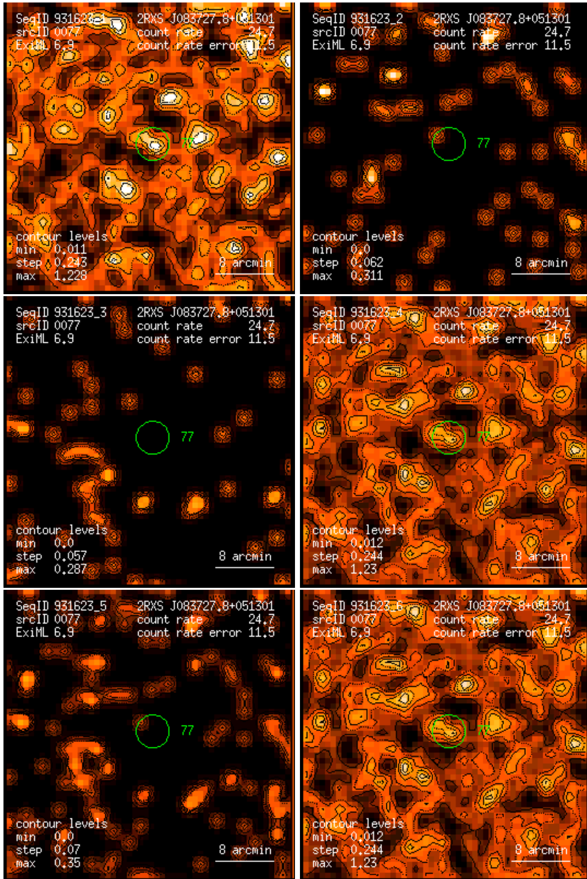
Figure 77: RASS 931623: detection 0077: band rate images, Gaussian filter: (1) PSPC channels 11 – 41, (2) 52 – 90, (3) 91 – 201, (4) 11 – 235, (5) 52 – 201, (6) 11 – 201. Broad band rates in counts/ks. Band rate contour levels in counts/ks/arcmin 2 .
