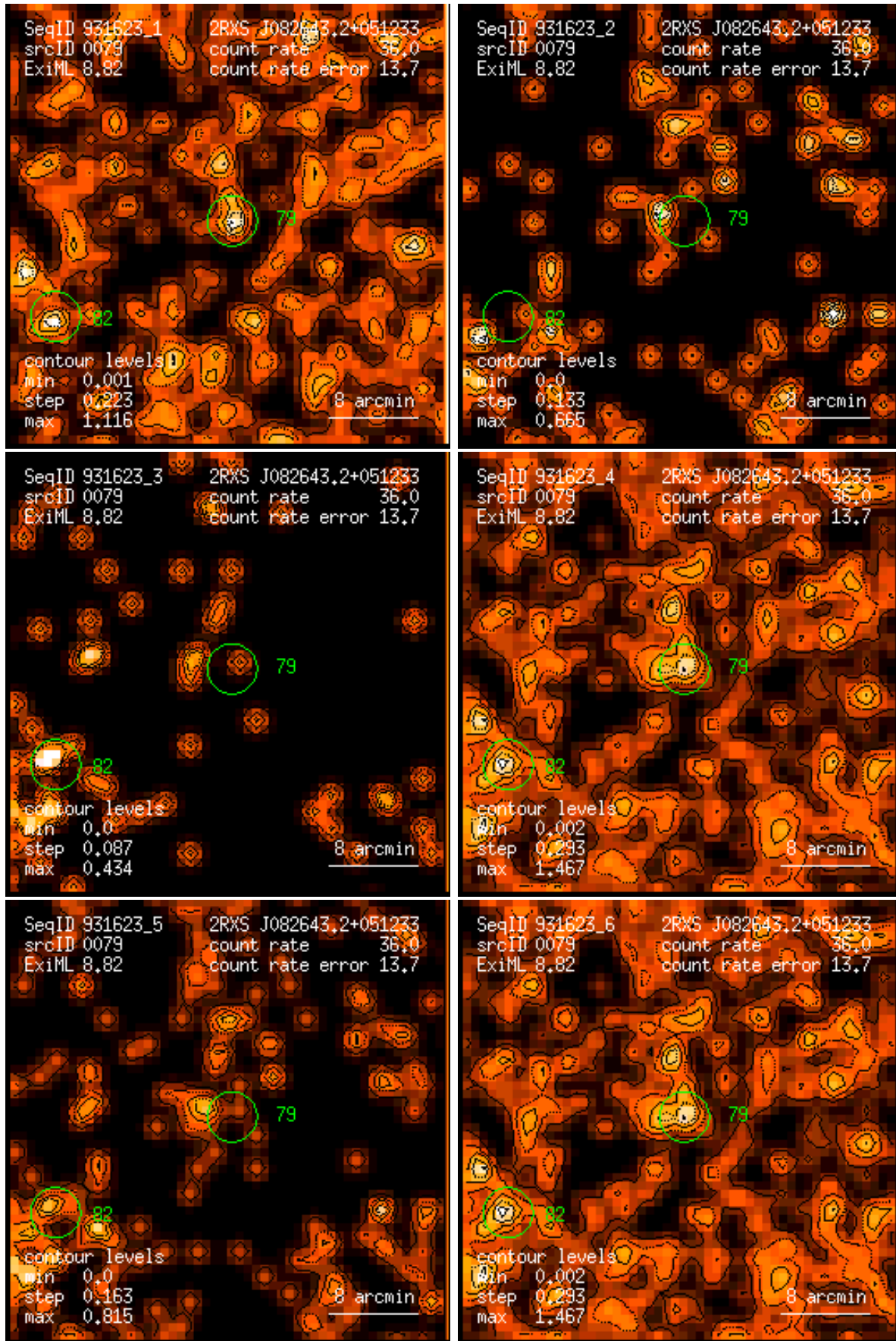
Figure 79: RASS 931623: detection 0079: band rate images, Gaussian filter: (1) PSPC channels 11 – 41, (2) 52 – 90, (3) 91 – 201, (4) 11 – 235, (5) 52 – 201, (6) 11 – 201. Broad band rates in counts/ks. Band rate contour levels in counts/ks/arcmin 2 .
