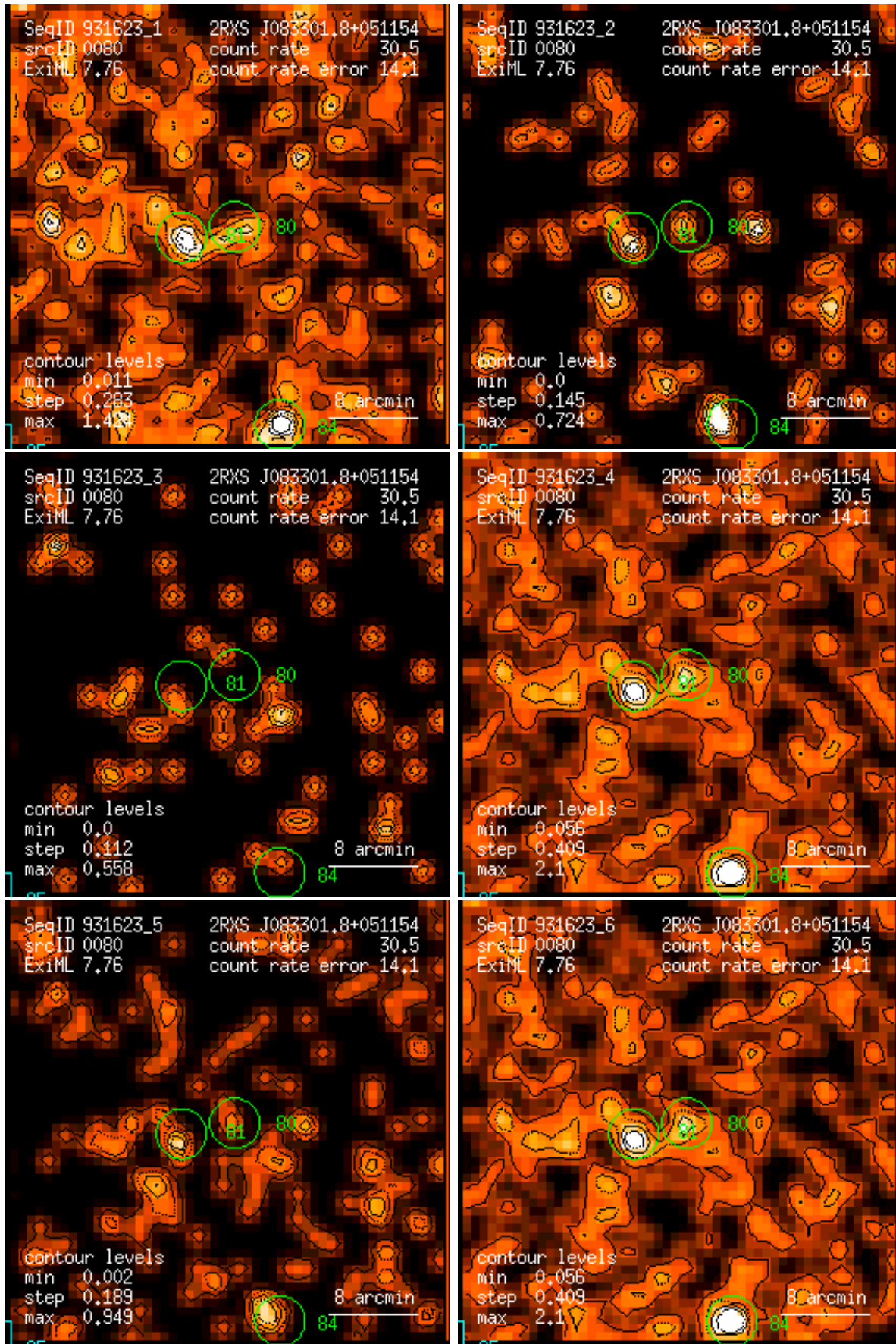
Figure 80: RASS 931623: detection 0080: band rate images, Gaussian filter: (1) PSPC channels 11 – 41, (2) 52 – 90, (3) 91 – 201, (4) 11 – 235, (5) 52 – 201, (6) 11 – 201. Broad band rates in counts/ks. Band rate contour levels in counts/ks/arcmin 2 .
